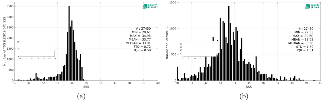
Figure 3: Histograms of SSS from TSG (LEGOS-DM) (a) and SMOS SSS L3 v335 - Monthly - 25 km (CATDS-CPDC) (b) considering all match-up pairs per bins of 0.1 over the Sea of Japan Pi-MEP region and for the full satellite product period.
