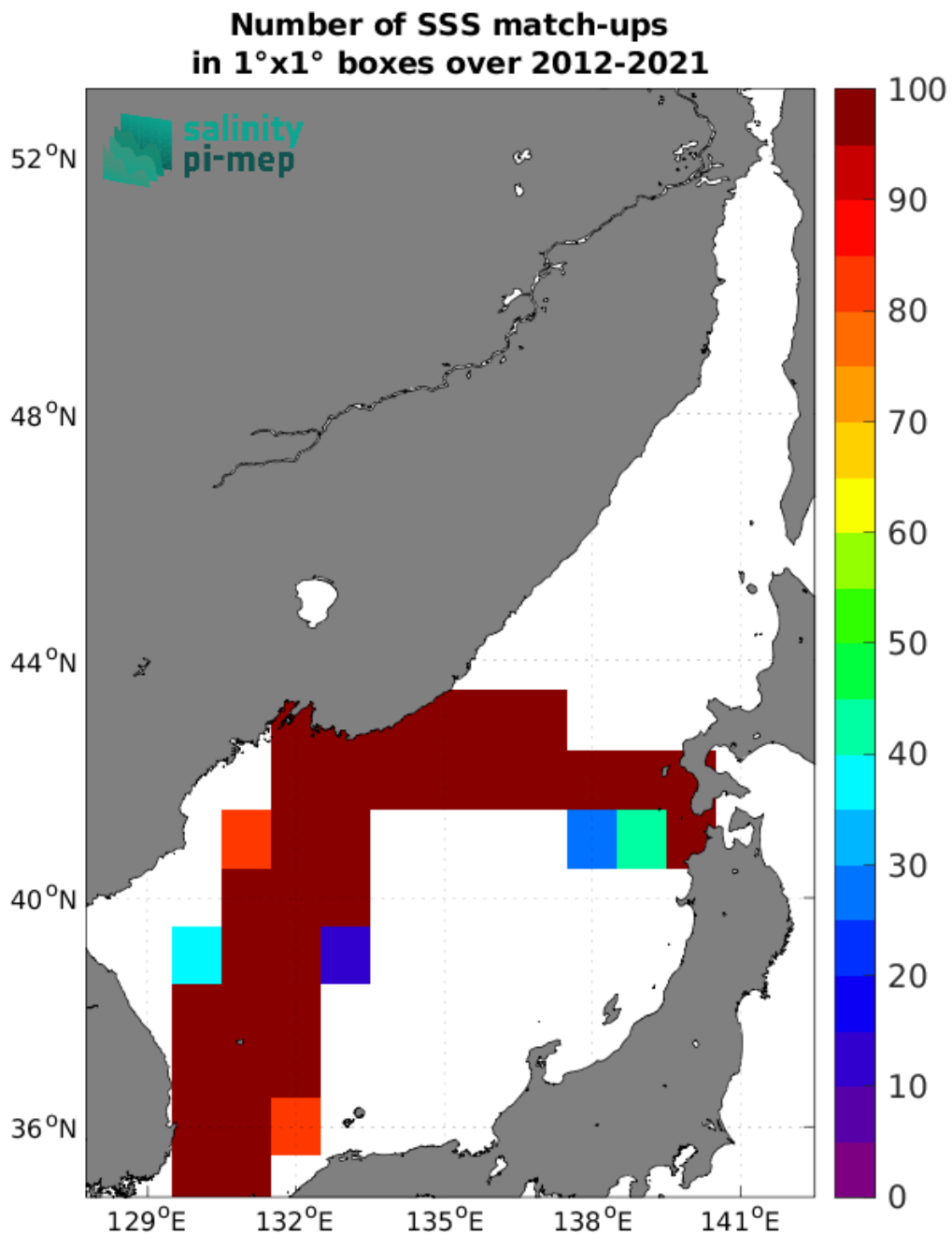
Figure 5: Number of SSS match-ups between TSG (LEGOS-DM) SSS and the SMOS SSS L3 v335 - Monthly - 25 km (CATDS-CPDC) SSS product for the Sea of Japan Pi-MEP region over 1°x1° boxes and for the full satellite product period.
