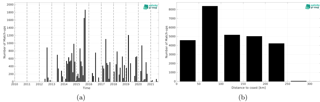
Figure 2: Number of match-ups between TSG (LEGOS-DM) and SMOS SSS L3 v335 - Monthly - 25 km (CATDS-CPDC) SSS as a function of time (a) and as function of the distance to coast (b) over the Sea of Japan Pi-MEP region and for the full satellite product period.
