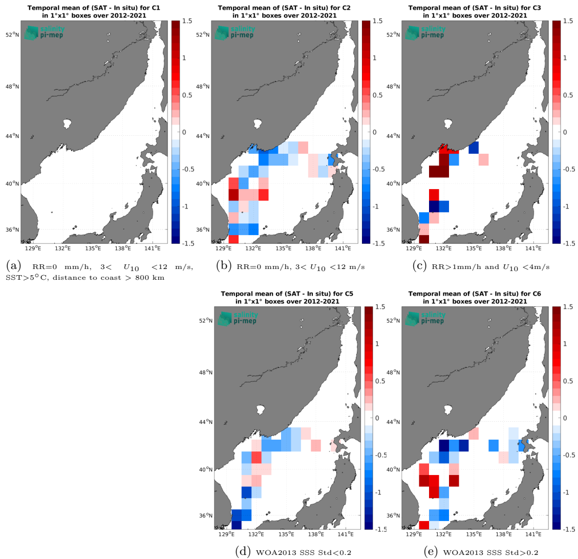
Figure 14: Temporal mean gridded over spatial boxes of size 1^\circ \times 1^\circ of \Delta\text{SSS} (SMOS SSS L3 v335 - Monthly - 25 km (CATDS-CPDC) - TSG (LEGOS-DM)) for 5 different subdatasets corresponding to: RR=0 mm/h, 3 < U_{10} < 12 m/s, SST > 5^\circ\text{C} , distance to coast > 800 km (a), RR=0 mm/h, 3 < U_{10} < 12 m/s (b), RR > 1 mm/h and U_{10} < 4 m/s (c), WOA2013 SSS Std < 0.2 (d), WOA2013 SSS Std > 0.2 (e).
