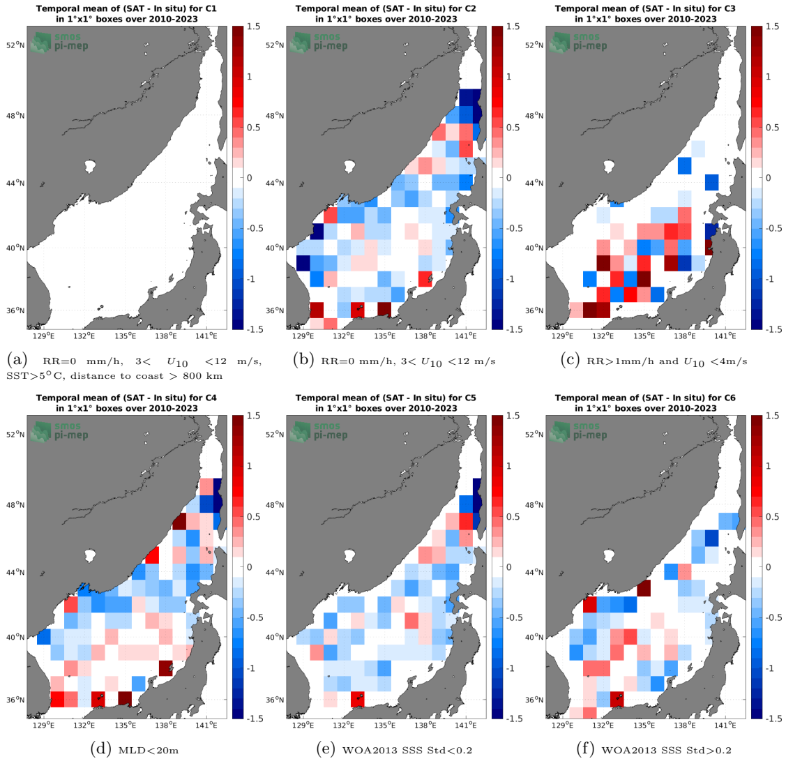
Figure 12: Temporal mean gridded over spatial boxes of size 1^\circ \times 1^\circ of \Delta\text{SSS} (SMOS SSS L3 v335 - Monthly - 25 km (CATDS-CPDC) - Argo) for 6 different subdatasets corresponding to: RR=0 mm/h, 3 < U_{10} < 12 m/s, SST > 5^\circ\text{C} , distance to coast > 800 km (a), RR=0 mm/h, 3 < U_{10} < 12 m/s (b), RR > 1 mm/h and U_{10} < 4 m/s (c), MLD < 20 m (d), WOA2013 SSS Std < 0.2 (e), WOA2013 SSS Std > 0.2 (f).
