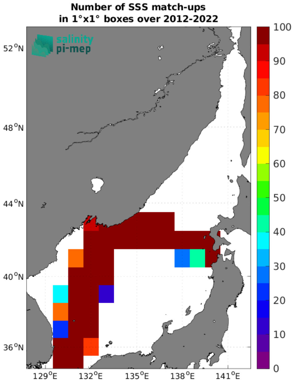
Figure 5: Number of SSS match-ups between TSG (LEGOS-DM) SSS and the SMOS SSS L3 v335 - 10 Days - 25 km (CATDS-CPDC) SSS product for the Sea of Japan Pi-MEP region over 1°x1° boxes and for the full satellite product period.
