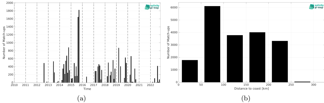
Figure 2: Number of match-ups between TSG (LEGOS-DM) and SMOS SSS L3 v335 - 10 Days - 25 km (CATDS-CPDC) SSS as a function of time (a) and as function of the distance to coast (b) over the Sea of Japan Pi-MEP region and for the full satellite product period.
