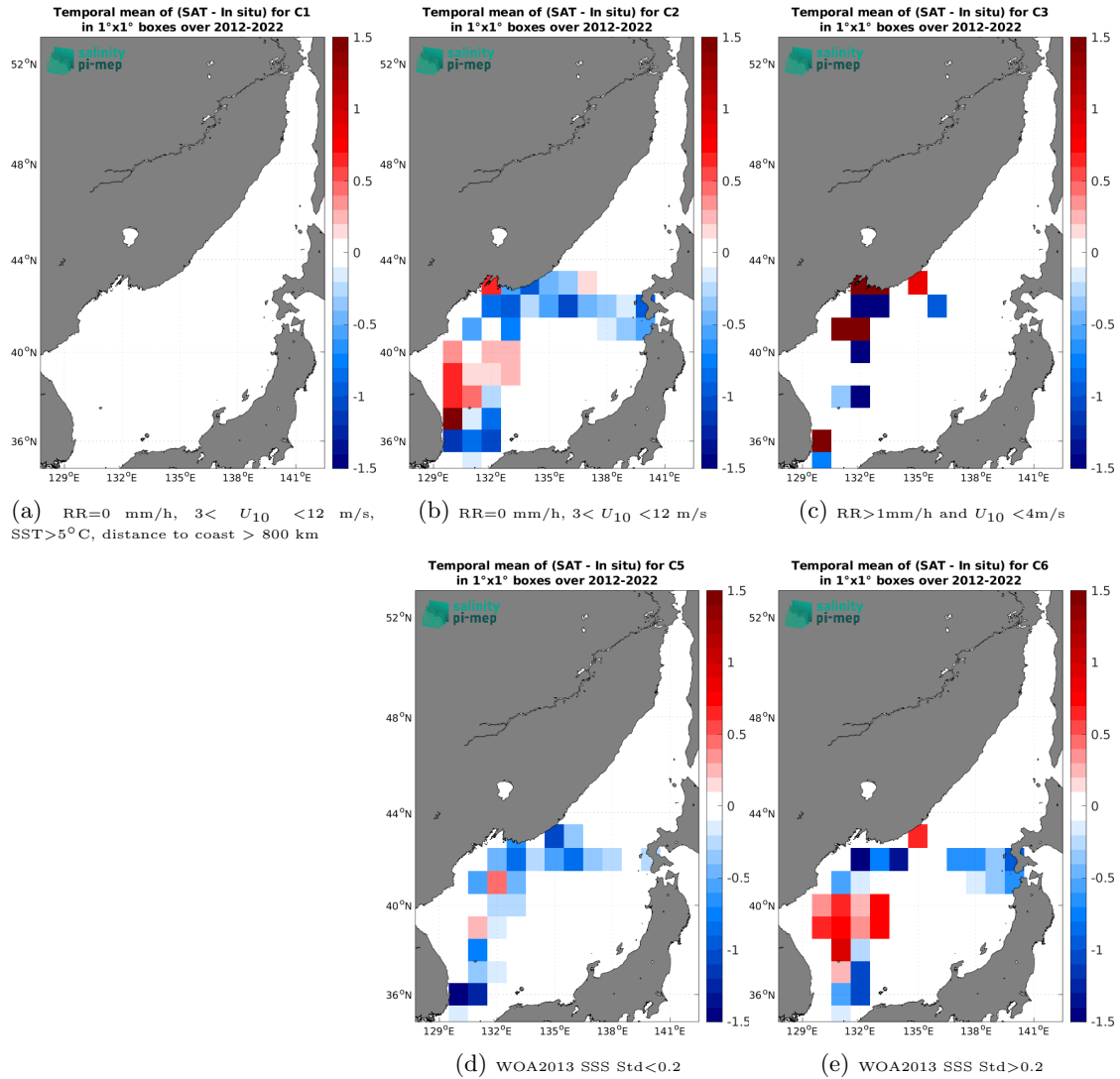
Figure 14: Temporal mean gridded over spatial boxes of size 1^\circ \times 1^\circ of \Delta\text{SSS} (SMOS SSS L3 v335 - 10 Days - 25 km (CATDS-CPDC) - TSG (LEGOS-DM)) for 5 different subdatasets corresponding to: RR=0 mm/h, 3 < U_{10} < 12 m/s, SST > 5^\circ\text{C} , distance to coast > 800 km (a), RR=0 mm/h, 3 < U_{10} < 12 m/s (b), RR > 1 mm/h and U_{10} < 4 m/s (c), WOA2013 SSS Std < 0.2 (d), WOA2013 SSS Std > 0.2 (e).
