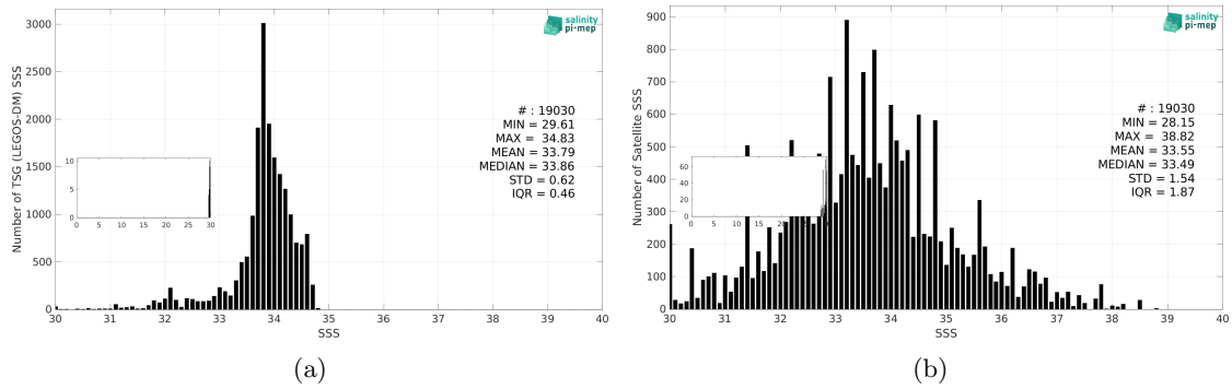
Figure 3: Histograms of SSS from TSG (LEGOS-DM) (a) and SMOS SSS L3 v335 - 10 Days - 25 km (CATDS-CPDC) (b) considering all match-up pairs per bins of 0.1 over the Sea of Japan Pi-MEP region and for the full satellite product period.
