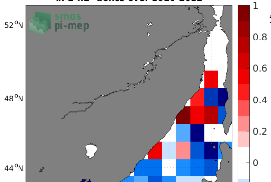
Temporal mean of (Sat - Argo) in 1°x1° boxes over 2010-2022
