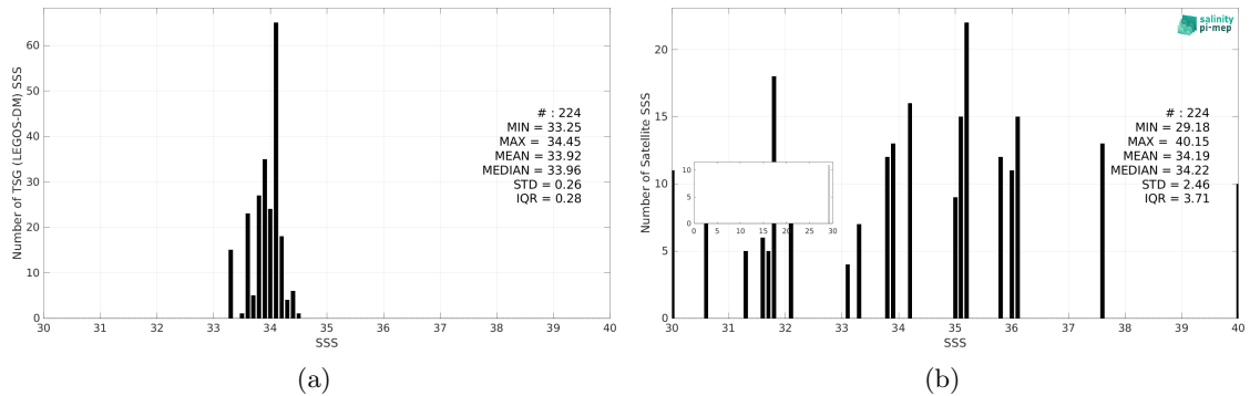
Figure 3: Histograms of SSS from TSG (LEGOS-DM) (a) and SMOS SSS L2Q v333 - 0.25 Deg (CATDS-CPDC) (b) considering all match-up pairs per bins of 0.1 over the Sea of Japan Pi-MEP region and for the full satellite product period.
