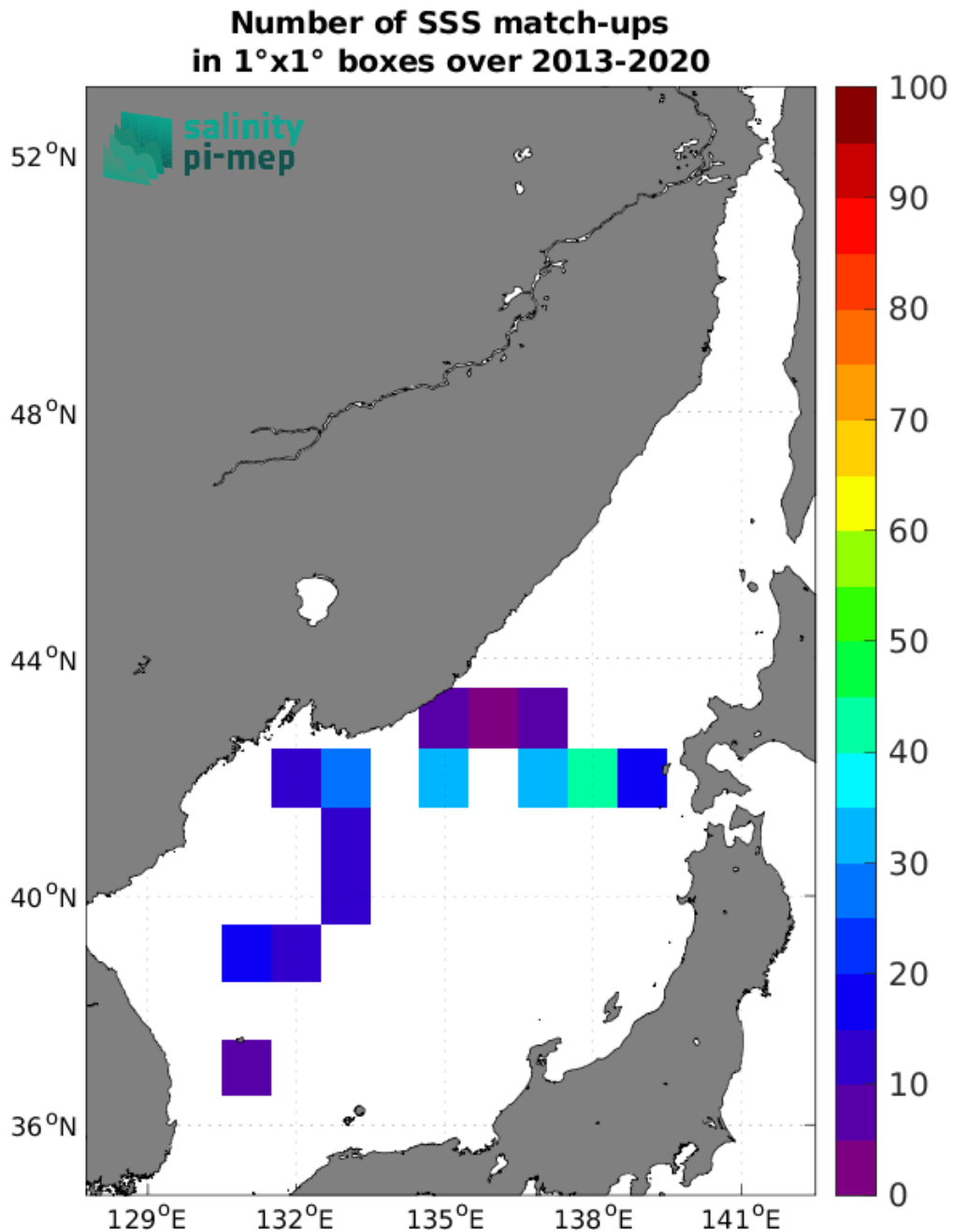
Figure 5: Number of SSS match-ups between TSG (LEGOS-DM) SSS and the SMOS SSS L2Q v333 - 0.25 Deg (CATDS-CPDC) SSS product for the Sea of Japan Pi-MEP region over 1°x1° boxes and for the full satellite product period.
