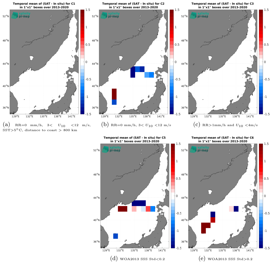
Figure 14: Temporal mean gridded over spatial boxes of size 1^\circ \times 1^\circ of \Delta\text{SSS} (SMOS SSS L2Q v333 - 0.25 Deg (CATDS-CPDC) - TSG (LEGOS-DM)) for 5 different subdatasets corresponding to: RR=0 mm/h, 3 < U_{10} < 12 m/s, SST > 5^\circ\text{C} , distance to coast > 800 km (a), RR=0 mm/h, 3 < U_{10} < 12 m/s (b), RR > 1\text{mm/h} and U_{10} < 4\text{m/s} (c), WOA2013 SSS Std < 0.2 (d), WOA2013 SSS Std > 0.2 (e).
