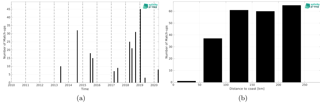
Figure 2: Number of match-ups between TSG (LEGOS-DM) and SMOS SSS L2Q v333 - 0.25 Deg (CATDS-CPDC) SSS as a function of time (a) and as function of the distance to coast (b) over the Sea of Japan Pi-MEP region and for the full satellite product period.
