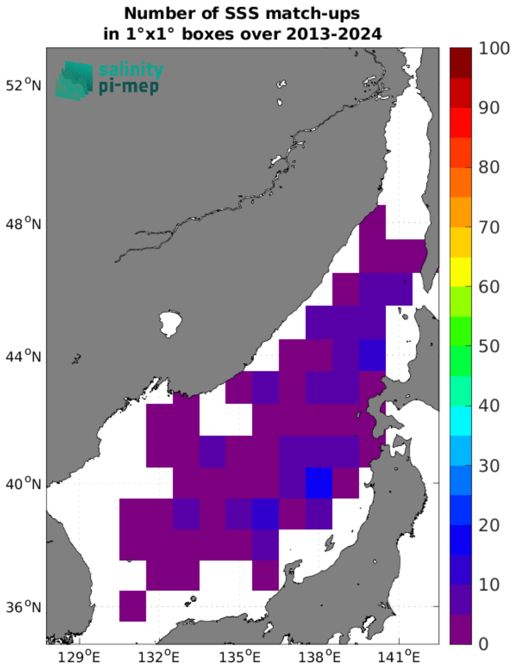
Figure 5: Number of SSS match-ups between Argo SSS and the SMOS SSS L2Q v333 - 0.25 Deg (CATDS-CPDC) SSS product for the Sea of Japan Pi-MEP region over 1°x1° boxes and for the full satellite product period.
