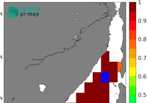
Temporal STD of (Sat - Argo) in 1°x1° boxes over 2013-2024
