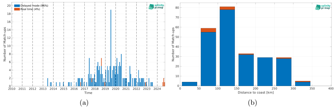
Figure 2: Number of match-ups between Argo and SMOS SSS L2Q v333 - 0.25 Deg (CATDS-CPDC) SSS as a function of time (a) and as function of the distance to coast (b) over the Sea of Japan Pi-MEP region and for the full satellite product period.
