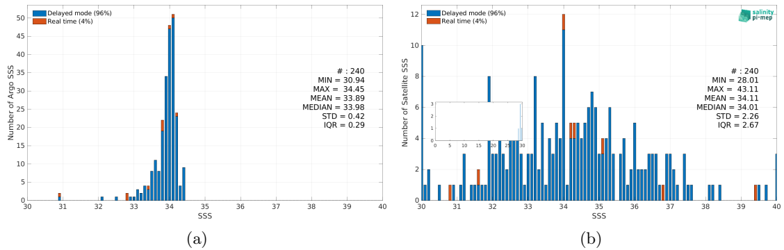
Figure 3: Histograms of SSS from Argo (a) and SMOS SSS L2Q v333 - 0.25 Deg (CATDS-CPDC) (b) considering all match-up pairs per bins of 0.1 over the Sea of Japan Pi-MEP region and for the full satellite product period.
