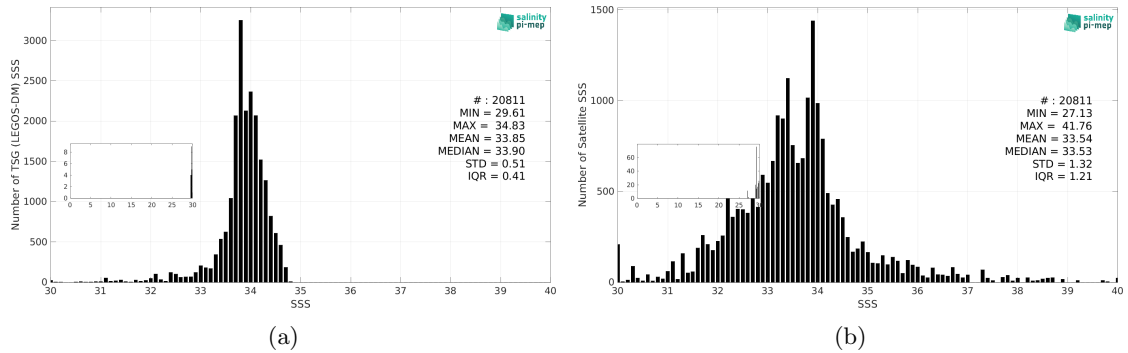
Figure 3: Histograms of SSS from TSG (LEGOS-DM) (a) and SMOS SSS L3 v332 - 9 Days (CATDS-CPDC) (b) considering all match-up pairs per bins of 0.1 over the Sea of Japan Pi-MEP region and for the full satellite product period.
