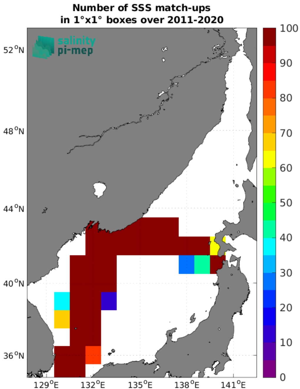
Figure 5: Number of SSS match-ups between TSG (LEGOS-DM) SSS and the SMOS SSS L3 v332 - 9 Days (CATDS-CPDC) SSS product for the Sea of Japan Pi-MEP region over 1°x1° boxes and for the full satellite product period.
