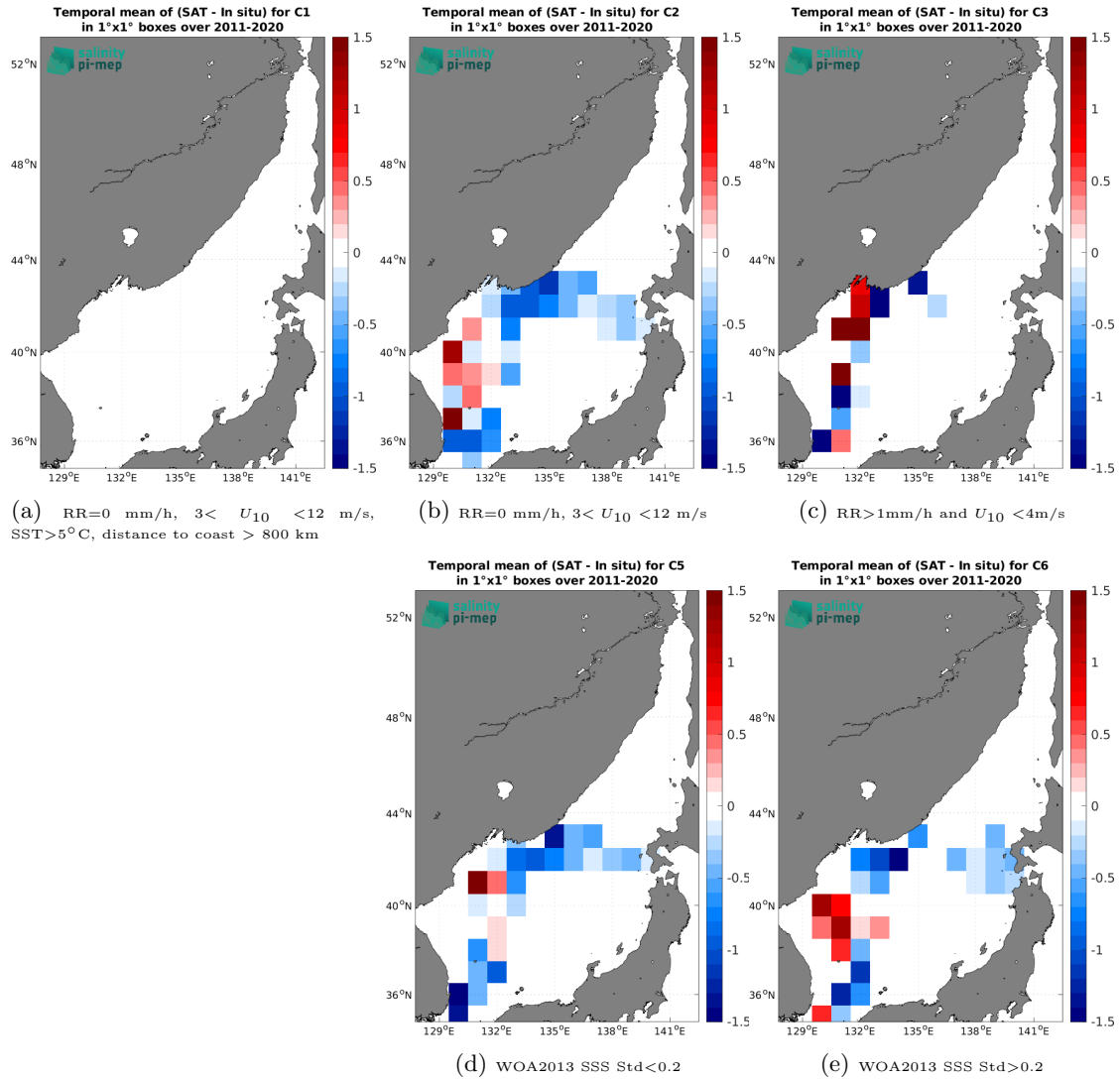
Figure 14: Temporal mean gridded over spatial boxes of size 1^\circ \times 1^\circ of \Delta\text{SSS} (SMOS SSS L3 v332 - 9 Days (CATDS-CPDC) - TSG (LEGOS-DM)) for 5 different subdatasets corresponding to: RR=0 mm/h, 3 < U_{10} < 12 m/s, SST > 5^\circ\text{C} , distance to coast > 800 km (a), RR=0 mm/h, 3 < U_{10} < 12 m/s (b), RR > 1\text{mm/h} and U_{10} < 4\text{m/s} (c), WOA2013 SSS Std < 0.2 (d), WOA2013 SSS Std > 0.2 (e).
