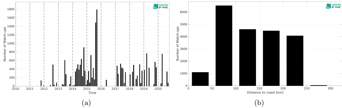
Figure 2: Number of match-ups between TSG (LEGOS-DM) and SMOS SSS L3 v332 - 9 Days (CATDS-CPDC) SSS as a function of time (a) and as function of the distance to coast (b) over the Sea of Japan Pi-MEP region and for the full satellite product period.
