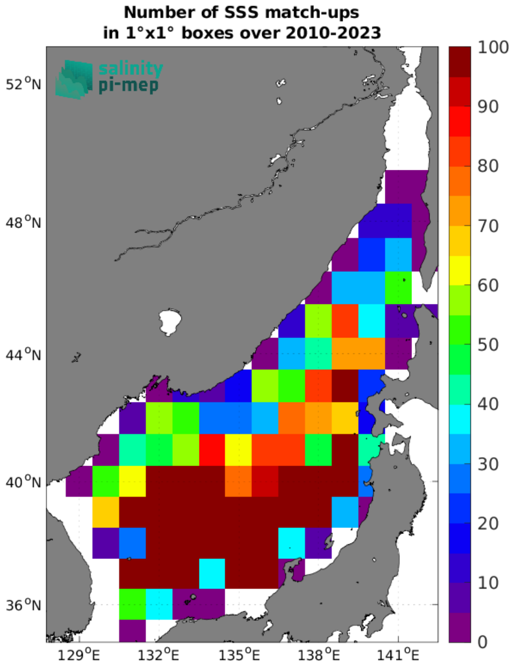
Figure 4: Number of SSS match-ups between Argo SSS and the SMOS SSS L3 v332 - 9 Days (CATDS-CPDC) SSS product for the Sea of Japan Pi-MEP region over 1°x1° boxes and for the full satellite product period.
