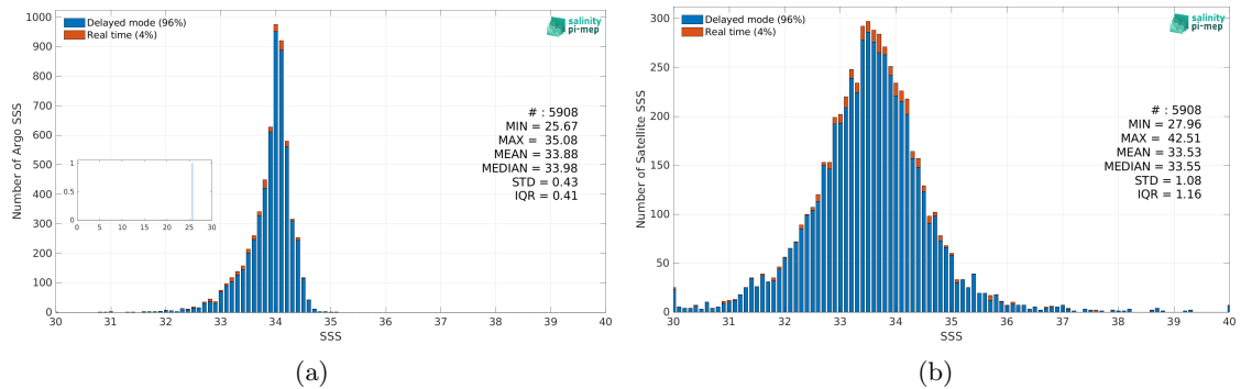
Figure 2: Histograms of SSS from Argo (a) and SMOS SSS L3 v332 - 9 Days (CATDS-CPDC) (b) considering all match-up pairs per bins of 0.1 over the Sea of Japan Pi-MEP region and for the full satellite product period.
