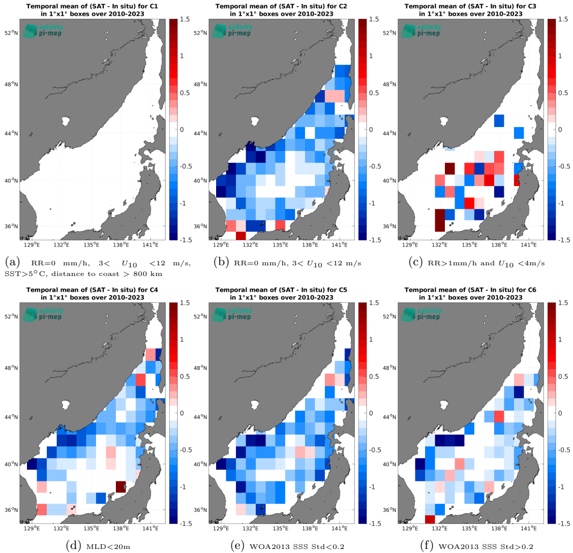
Figure 12: Temporal mean gridded over spatial boxes of size 1^\circ \times 1^\circ of \Delta SSS (SMOS SSS L3 v332 - 9 Days (CATDS-CPDC) - Argo) for 6 different subdatasets corresponding to: RR=0 mm/h, 3 < U_{10} < 12 m/s, SST > 5°C, distance to coast > 800 km (a), RR=0 mm/h, 3 < U_{10} < 12 m/s (b), RR > 1mm/h and U_{10} < 4 m/s (c), MLD < 20m (d), WOA2013 SSS Std < 0.2 (e), WOA2013 SSS Std > 0.2 (f).
