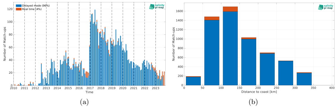
Figure 1: Number of match-ups between Argo and SMOS SSS L3 v332 - 9 Days (CATDS-CPDC) SSS as a function of time (a) and as function of the distance to coast (b) over the Sea of Japan Pi-MEP region and for the full satellite product period.
