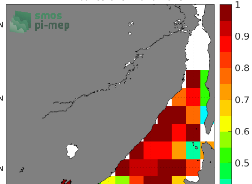
Temporal STD of (Sat - Argo) in 1°x1° boxes over 2010-2023
