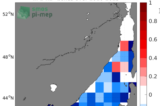
Temporal mean of (Sat - Argo) in 1°x1° boxes over 2010-2023
