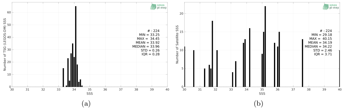
Figure 2: Histograms of SSS from TSG (LEGOS-DM) (a) and SMOS SSS L2Q v331 - 0.25 Deg (CATDS-CPDC) (b) considering all match-up pairs per bins of 0.1 over the Sea of Japan Pi-MEP region and for the full satellite product period.
