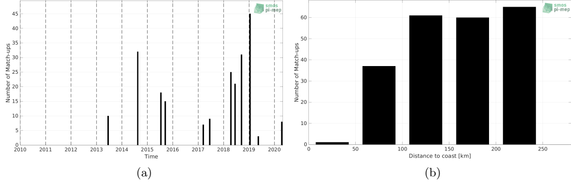
Figure 1: Number of match-ups between TSG (LEGOS-DM) and SMOS SSS L2Q v331 - 0.25 Deg (CATDS-CPDC) SSS as a function of time (a) and as function of the distance to coast (b) over the Sea of Japan Pi-MEP region and for the full satellite product period.
