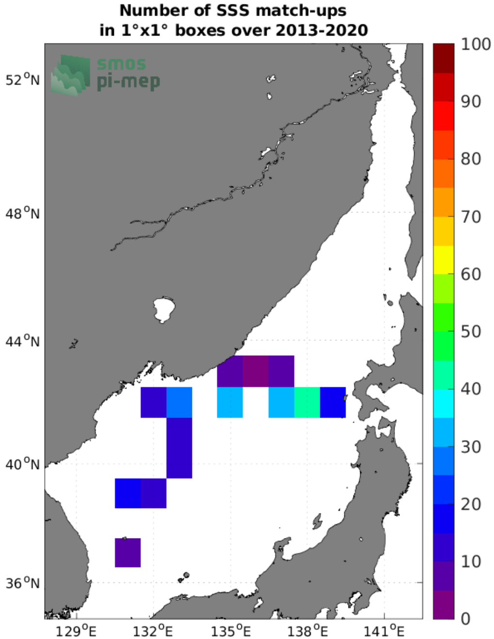
Figure 4: Number of SSS match-ups between TSG (LEGOS-DM) SSS and the SMOS SSS L2Q v331 - 0.25 Deg (CATDS-CPDC) SSS product for the Sea of Japan Pi-MEP region over 1°x1° boxes and for the full satellite product period.
