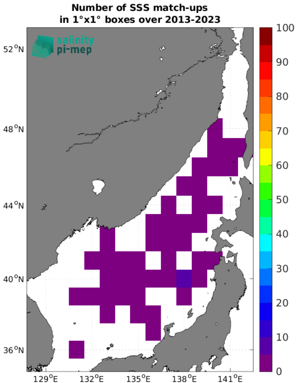
Figure 4: Number of SSS match-ups between Argo SSS and the SMOS SSS L2Q v331 - 0.25 Deg (CATDS-CPDC) SSS product for the Sea of Japan Pi-MEP region over 1°x1° boxes and for the full satellite product period.
