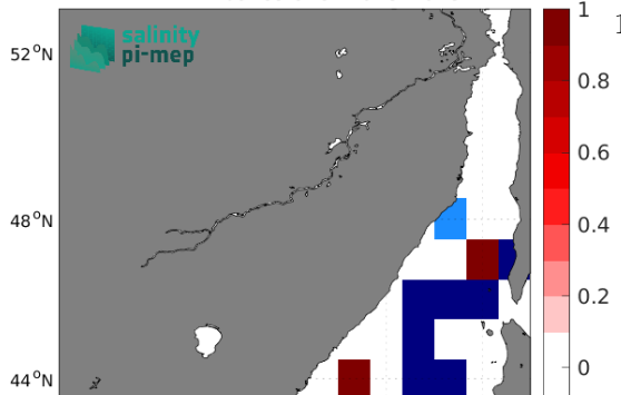
Temporal mean of (Sat - Argo) in 1°x1° boxes over 2013-2023
