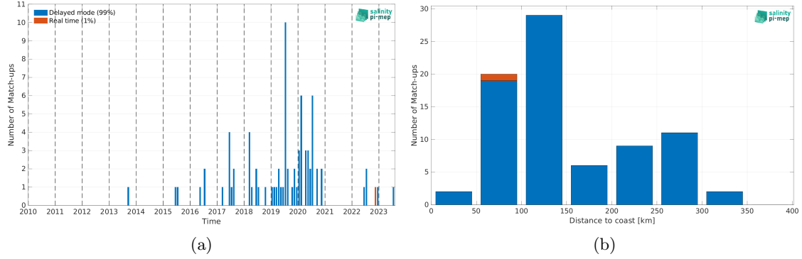
Figure 1: Number of match-ups between Argo and SMOS SSS L2Q v331 - 0.25 Deg (CATDS-CPDC) SSS as a function of time (a) and as function of the distance to coast (b) over the Sea of Japan Pi-MEP region and for the full satellite product period.
