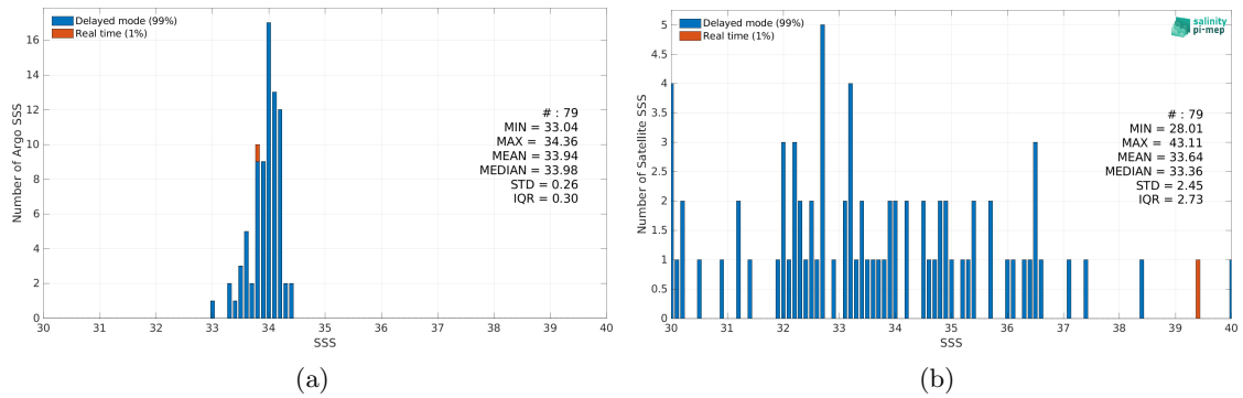
Figure 2: Histograms of SSS from Argo (a) and SMOS SSS L2Q v331 - 0.25 Deg (CATDS-CPDC) (b) considering all match-up pairs per bins of 0.1 over the Sea of Japan Pi-MEP region and for the full satellite product period.
