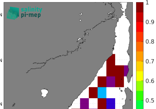
Temporal STD of (Sat - Argo) in 1°x1° boxes over 2013-2023
