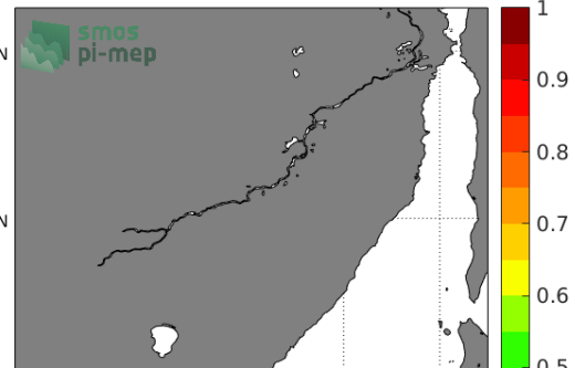
Temporal STD of (Sat - TSG (LEGOS-DM)) in 1°x1° boxes over 2013-2019
