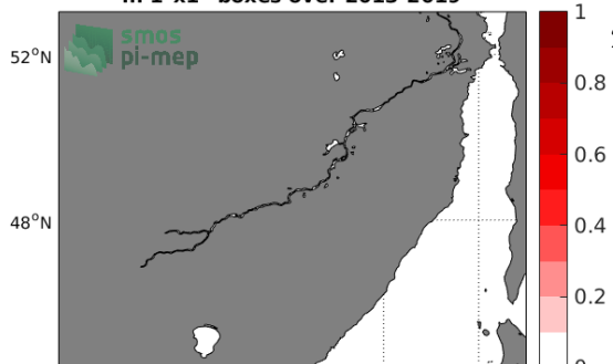
Temporal mean of (Sat - TSG (LEGOS-DM)) in 1°x1° boxes over 2013-2019
