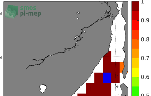
Temporal STD of (Sat - Argo) in 1°x1° boxes over 2013-2021
