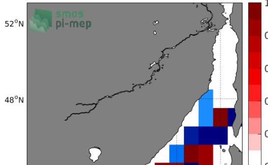
Temporal mean of (Sat - Argo) in 1°x1° boxes over 2013-2021
