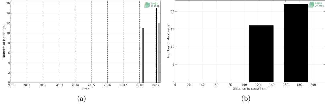
Figure 1: Number of match-ups between TSG (LEGOS-DM) and SMOS SSS L2Q v321 - 0.25 Deg (CATDS-CPDC) SSS as a function of time (a) and as function of the distance to coast (b) over the Sea of Japan Pi-MEP region and for the full satellite product period.
