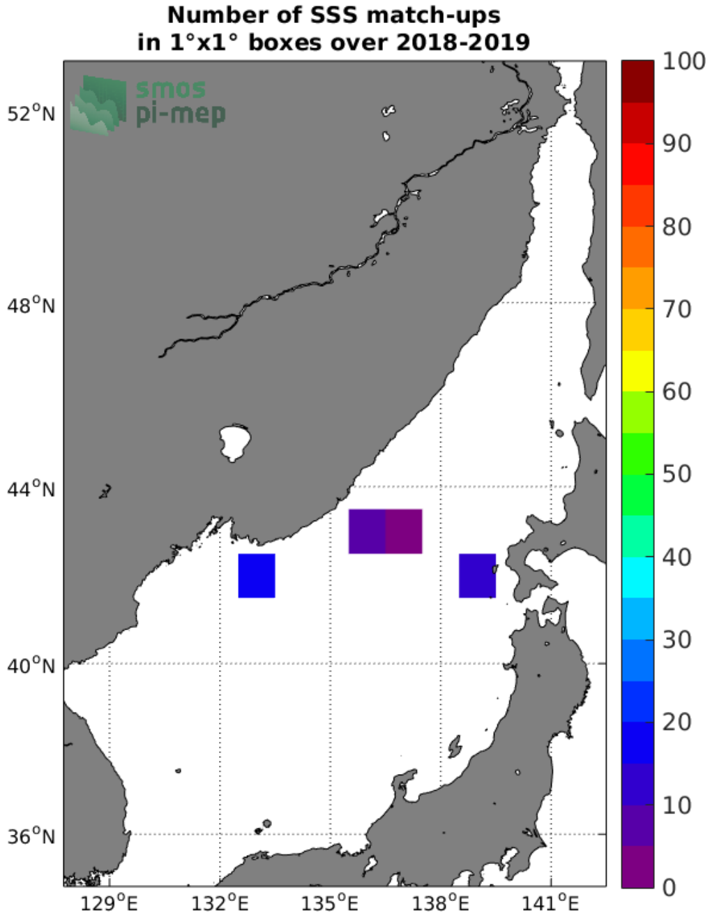
Figure 4: Number of SSS match-ups between TSG (LEGOS-DM) SSS and the SMOS SSS L2Q v321 - 0.25 Deg (CATDS-CPDC) SSS product for the Sea of Japan Pi-MEP region over 1°x1° boxes and for the full satellite product period.
