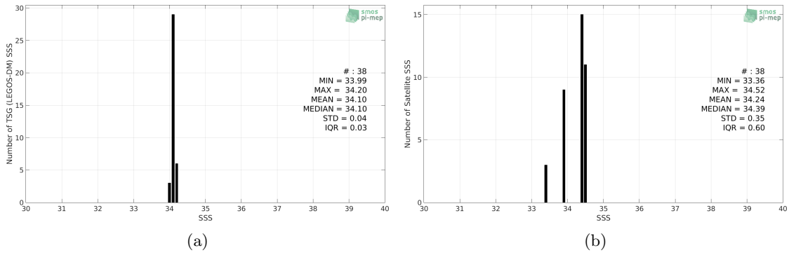
Figure 2: Histograms of SSS from TSG (LEGOS-DM) (a) and SMOS SSS L2Q v321 - 0.25 Deg (CATDS-CPDC) (b) considering all match-up pairs per bins of 0.1 over the Sea of Japan Pi-MEP region and for the full satellite product period.
