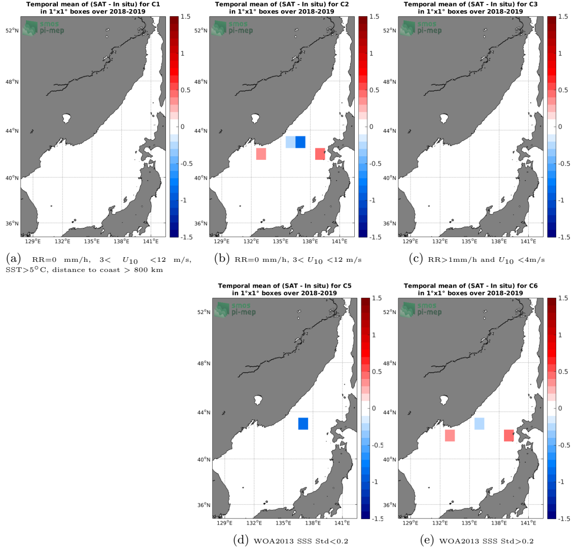
Figure 12: Temporal mean gridded over spatial boxes of size 1^\circ \times 1^\circ of \Delta\text{SSS} (SMOS SSS L2Q v321 - 0.25 Deg (CATDS-CPDC) - TSG (LEGOS-DM)) for 5 different subdatasets corresponding to: RR=0 mm/h, 3 < U_{10} < 12 m/s, SST > 5^\circ\text{C} , distance to coast > 800 km (a), RR=0 mm/h, 3 < U_{10} < 12 m/s (b), RR > 1 mm/h and U_{10} < 4 m/s (c), WOA2013 SSS Std < 0.2 (d), WOA2013 SSS Std > 0.2 (e).
