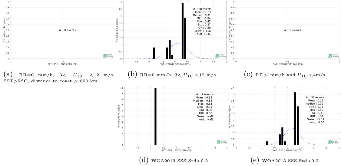
Figure 13: Normalized histogram of \Delta\text{SSS} (SMOS SSS L2Q v321 - 0.25 Deg (CATDS-CPDC) - TSG (LEGOS-DM)) for 5 different subdatasets corresponding to: RR=0 mm/h, 3 < U_{10} < 12 m/s, SST > 5^\circ\text{C} , distance to coast > 800 km (a), RR=0 mm/h, 3 < U_{10} < 12 m/s (b), RR > 1\text{mm/h} and U_{10} < 4\text{m/s} (c), WOA2013 SSS Std < 0.2 (d), WOA2013 SSS Std > 0.2 (e).
