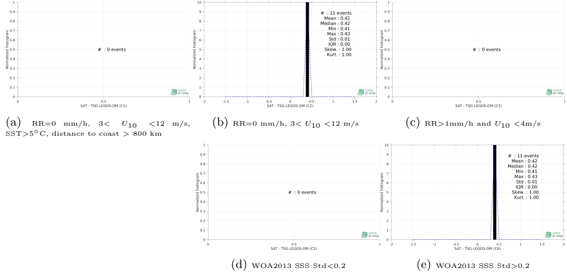
Figure 13: Normalized histogram of \Delta\text{SSS} (SMOS-L3-CATDS-CPDC-V321-L2Q - TSG-LEGOS-DM) for 5 different subdatasets corresponding to: RR=0 mm/h, 3 < U_{10} < 12 m/s, SST >5^{\circ}\text{C} , distance to coast > 800 km (a), RR=0 mm/h, 3 < U_{10} < 12 m/s (b), RR>1\text{mm/h} and U_{10} < 4\text{m/s} (c), WOA2013 SSS Std <0.2 (d), WOA2013 SSS Std >0.2 (e).
