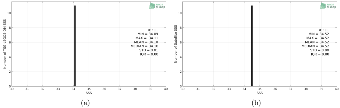
Figure 2: Histograms of SSS from TSG-LEGOS-DM (a) and SMOS-L3-CATDS-CPDC-V321-L2Q (b) considering all match-up pairs per bins of 0.1 over the Sea of Japan Pi-MEP region and for the full satellite product period.
