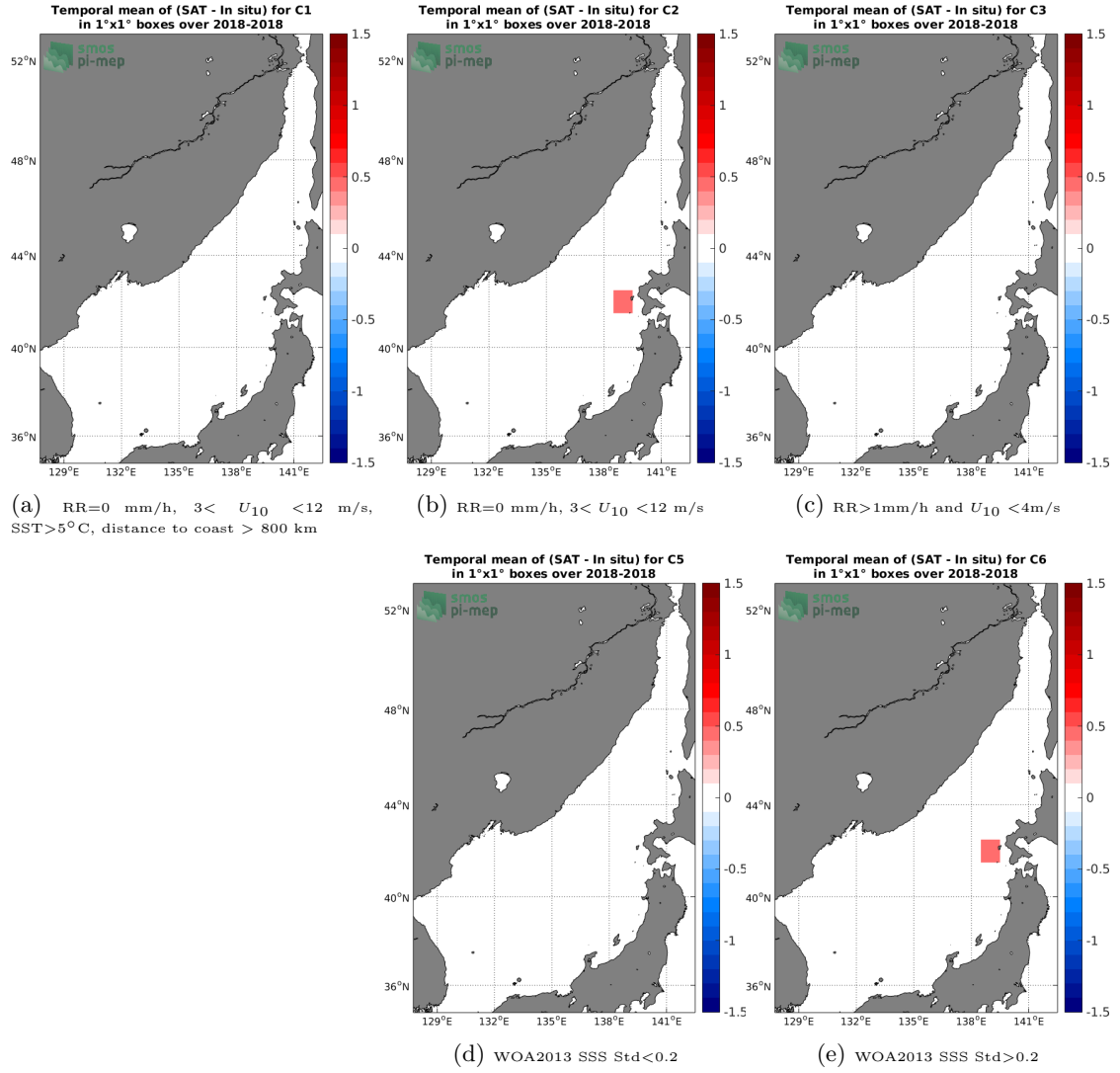
Figure 12: Temporal mean gridded over spatial boxes of size 1°x1° of \Delta SSS (SMOS-L3-CATDS-CPDC-V321-L2Q - TSG-LEGOS-DM) for 5 different subdatasets corresponding to: RR=0 mm/h, 3 < U_{10} < 12 m/s, SST>5°C, distance to coast > 800 km (a), RR=0 mm/h, 3 < U_{10} < 12 m/s (b), RR>1 mm/h and U_{10} < 4 m/s (c), WOA2013 SSS Std<0.2 (d), WOA2013 SSS Std>0.2 (e).
