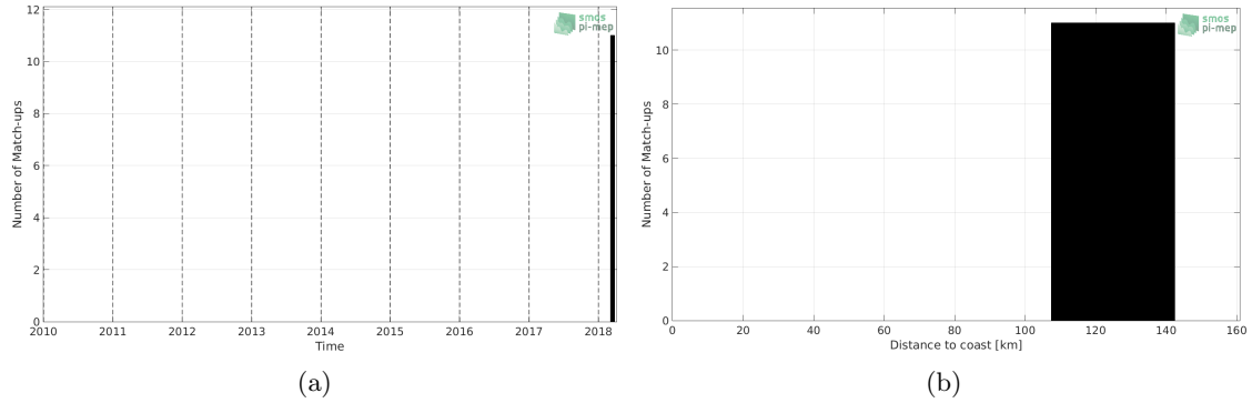
Figure 1: Number of match-ups between TSG-LEGOS-DM and SMOS-L3-CATDS-CPDC-V321-L2Q SSS as a function of time (a) and as function of the distance to coast (b) over the Sea of Japan Pi-MEP region and for the full satellite product period.
