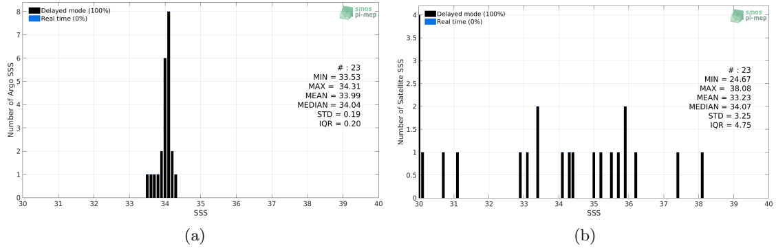
Figure 2: Histograms of SSS from Argos (a) and SMOS SSS L2Q v321 - 0.25 Deg (CATDS-CPDC) (b) considering all match-up pairs per bins of 0.1 over the Sea of Japan Pi-MEP region and for the full satellite product period.
