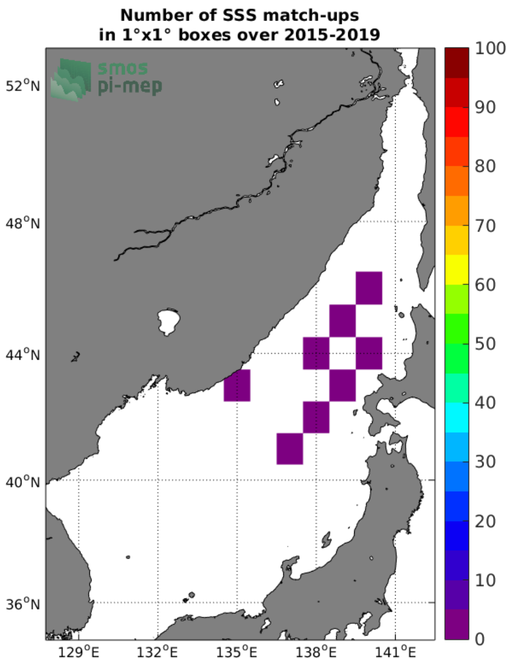
Figure 4: Number of SSS match-ups between Argo SSS and the SMOS-L3-CATDS-CPDC-V321-L2Q SSS product for the Sea of Japan Pi-MEP region over 1°x1° boxes and for the full satellite product period.
