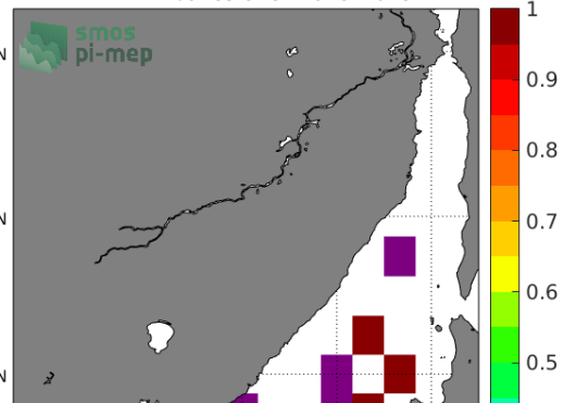
Temporal STD of (Sat - Argo) in 1°x1° boxes over 2015-2019
