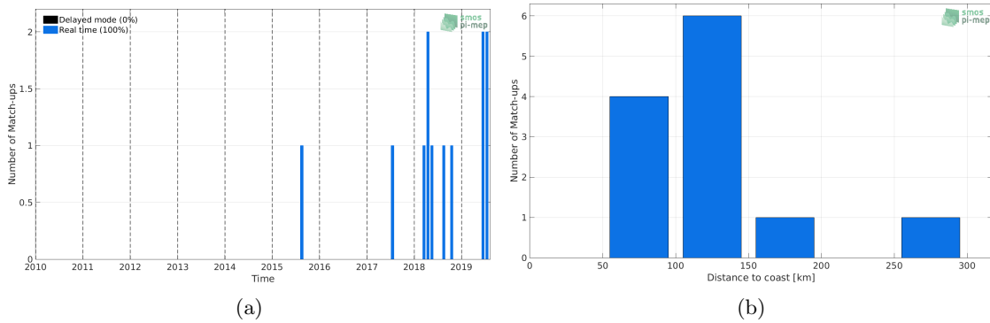
Figure 1: Number of match-ups between Argo and SMOS-L3-CATDS-CPDC-V321-L2Q SSS as a function of time (a) and as function of the distance to coast (b) over the Sea of Japan Pi-MEP region and for the full satellite product period.
