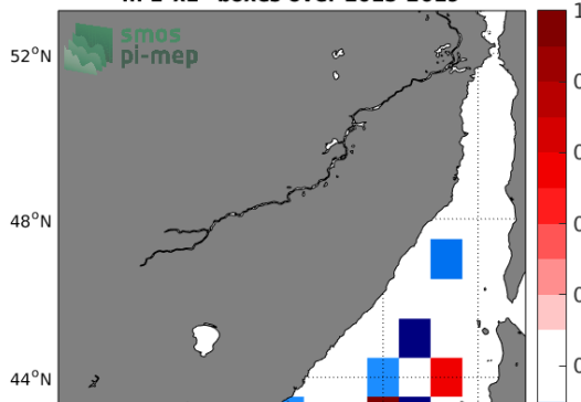
Temporal mean of (Sat - Argo) in 1°x1° boxes over 2015-2019
