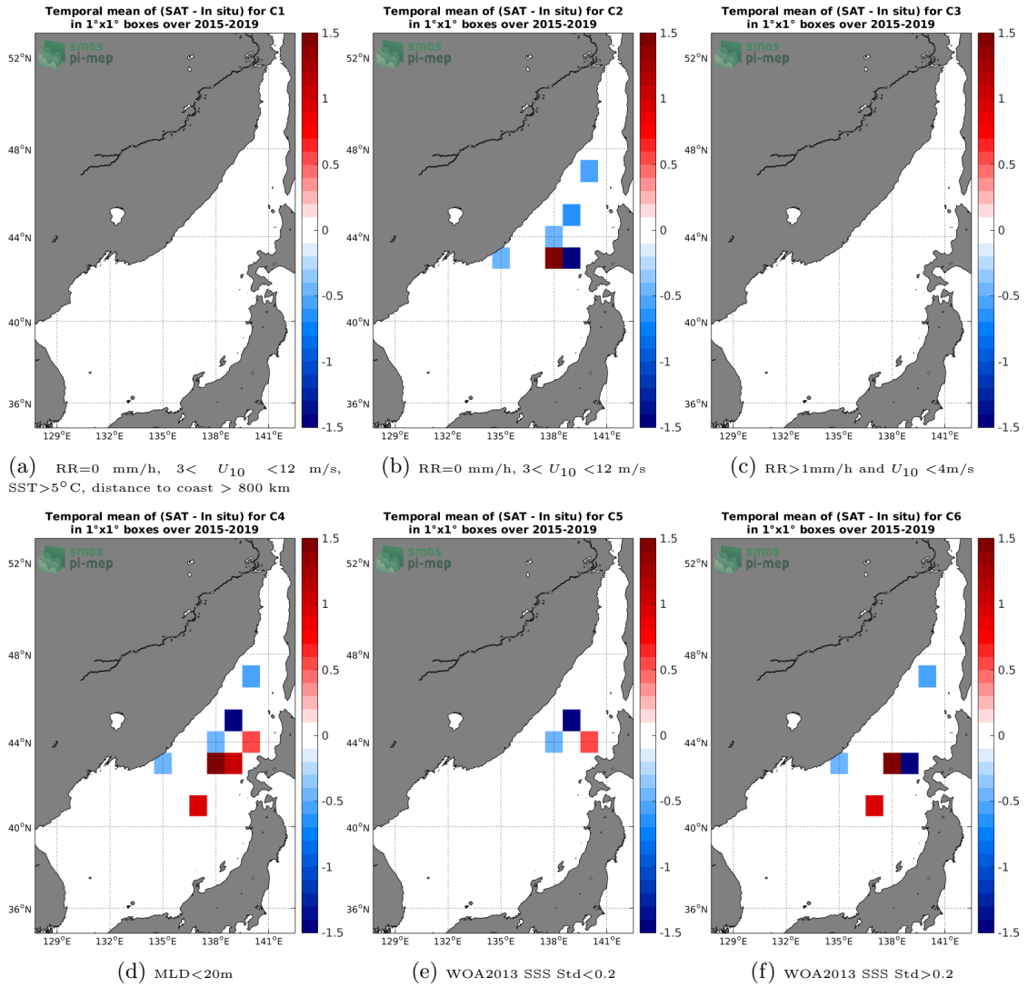
Figure 12: Temporal mean gridded over spatial boxes of size 1^{\circ} \times 1^{\circ} of \Delta SSS (SMOS-L3-CATDS-CPDC-V321-L2Q - Argo) for 6 different subdatasets corresponding to: RR=0 mm/h, 3 < U_{10} < 12 m/s, SST > 5^{\circ}C , distance to coast > 800 km (a), RR=0 mm/h, 3 < U_{10} < 12 m/s (b), RR > 1 mm/h and U_{10} < 4 m/s (c), MLD < 20 m (d), WOA2013 SSS Std < 0.2 (e), WOA2013 SSS Std > 0.2 (f).
