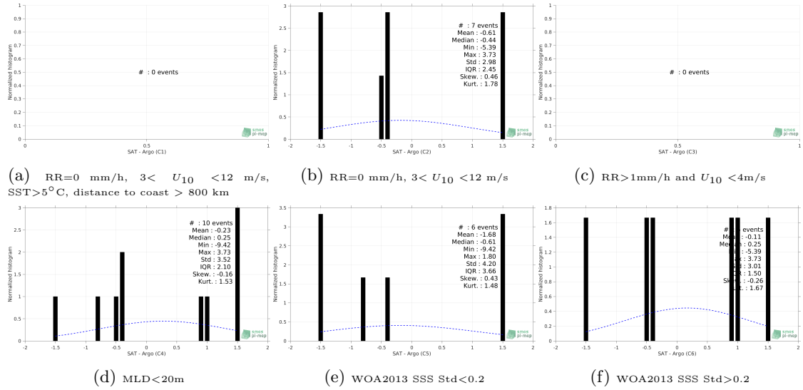
Figure 13: Normalized histogram of \Delta\text{SSS} (SMOS-L3-CATDS-CPDC-V321-L2Q - Argo) for 6 different subdatasets corresponding to: RR=0 mm/h, 3 < U_{10} < 12 m/s, SST >5^{\circ}\text{C} , distance to coast > 800 km (a), RR=0 mm/h, 3 < U_{10} < 12 m/s (b), RR >1 mm/h and U_{10} < 4 m/s (c), MLD <20 m (d), WOA2013 SSS Std <0.2 (e), WOA2013 SSS Std >0.2 (f).
