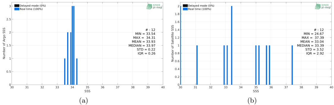
Figure 2: Histograms of SSS from Argo (a) and SMOS-L3-CATDS-CPDC-V321-L2Q (b) considering all match-up pairs per bins of 0.1 over the Sea of Japan Pi-MEP region and for the full satellite product period.
