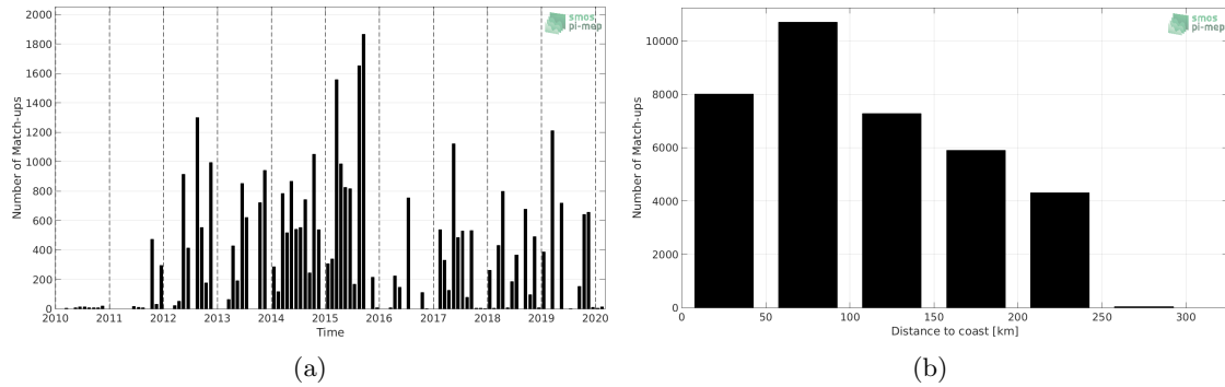
Figure 1: Number of match-ups between TSG (LEGOS-DM) and SMOS SSS L3 v317 - Monthly - 25 km (CATDS-CPDC) SSS as a function of time (a) and as function of the distance to coast (b) over the Sea of Japan Pi-MEP region and for the full satellite product period.
