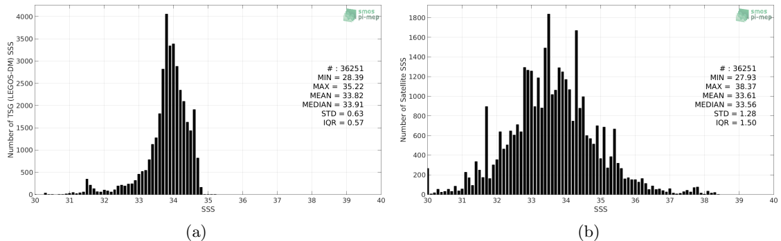
Figure 2: Histograms of SSS from TSG (LEGOS-DM) (a) and SMOS SSS L3 v317 - Monthly - 25 km (CATDS-CPDC) (b) considering all match-up pairs per bins of 0.1 over the Sea of Japan Pi-MEP region and for the full satellite product period.
