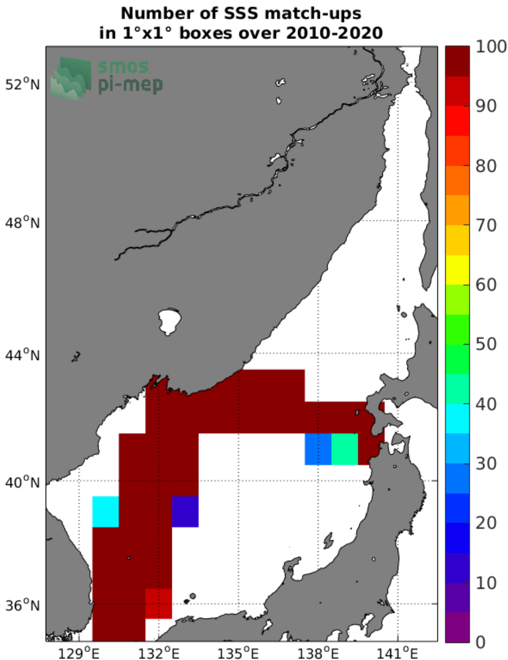
Figure 4: Number of SSS match-ups between TSG (LEGOS-DM) SSS and the SMOS SSS L3 v317 - Monthly - 25 km (CATDS-CPDC) SSS product for the Sea of Japan Pi-MEP region over 1°x1° boxes and for the full satellite product period.
