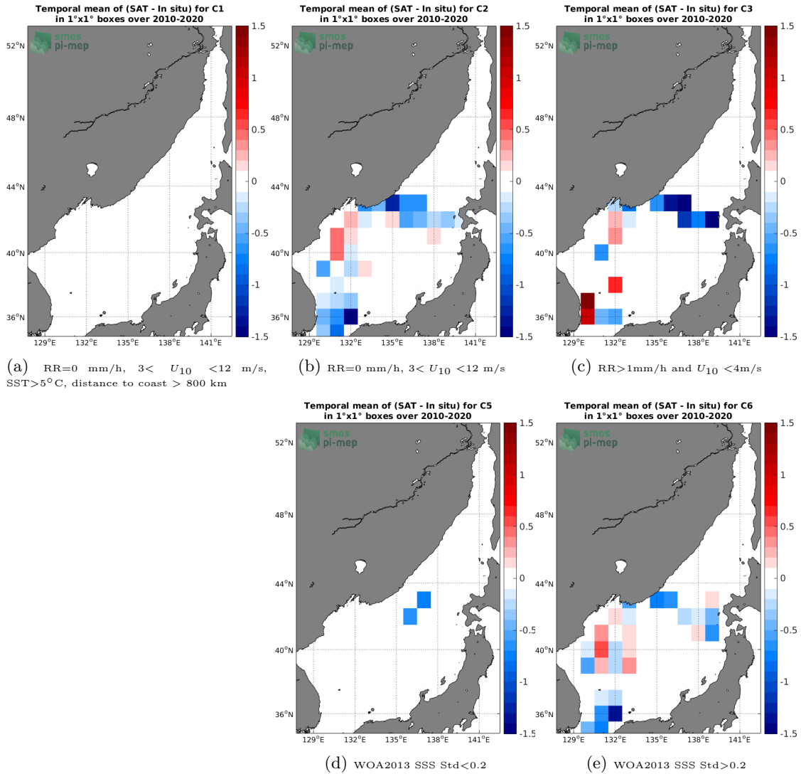
Figure 12: Temporal mean gridded over spatial boxes of size 1^\circ \times 1^\circ of \Delta SSS (SMOS SSS L3 v317 - Monthly - 25 km (CATDS-CPDC) - TSG (LEGOS-DM)) for 5 different subdatasets corresponding to:RR=0 mm/h, 3 < U_{10} < 12 m/s, SST>5°C, distance to coast > 800 km (a), RR=0 mm/h, 3 < U_{10} < 12 m/s (b), RR>1mm/h and U_{10} < 4 m/s (c), WOA2013 SSS Std<0.2 (d), WOA2013 SSS Std>0.2 (e).
