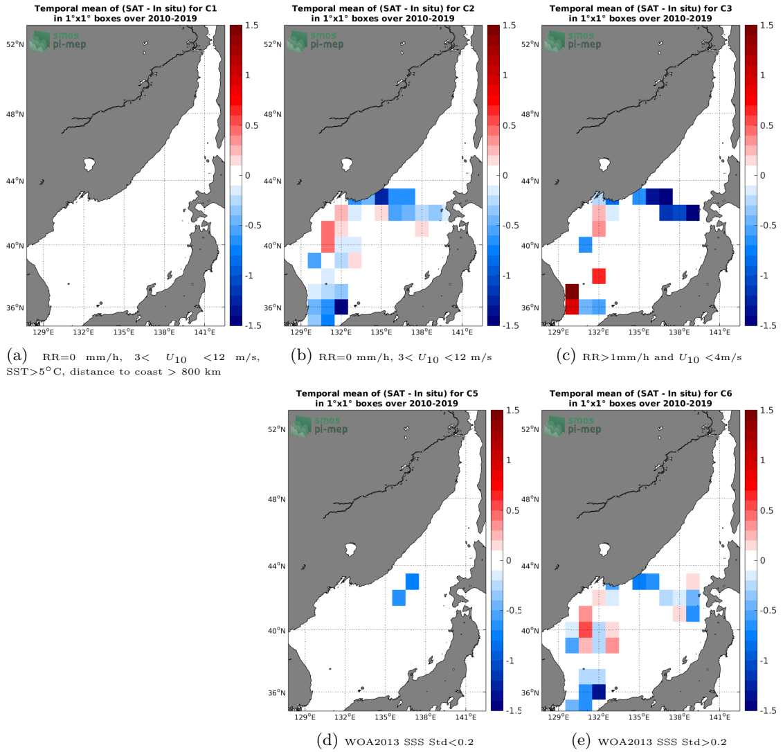
Figure 12: Temporal mean gridded over spatial boxes of size 1°x1° of \Delta\text{SSS} (SMOS L3 v317 - Monthly - 25 km (CATDS-CPDC) - TSG-LEGOS-DM) for 5 different subdatasets corresponding to: RR=0 mm/h, 3 < U_{10} < 12 m/s, SST > 5^\circ\text{C} , distance to coast > 800 km (a), RR=0 mm/h, 3 < U_{10} < 12 m/s (b), RR > 1 mm/h and U_{10} < 4 m/s (c), WOA2013 SSS Std < 0.2 (d), WOA2013 SSS Std > 0.2 (e).
