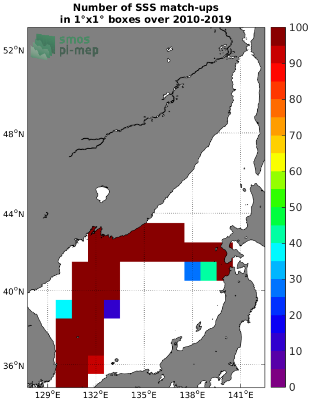
Figure 4: Number of SSS match-ups between TSG-LEGOS-DM SSS and the SMOS L3 v317 - Monthly - 25 km (CATDS-CPDC) SSS product for the Sea of Japan Pi-MEP region over 1°x1° boxes and for the full satellite product period.
