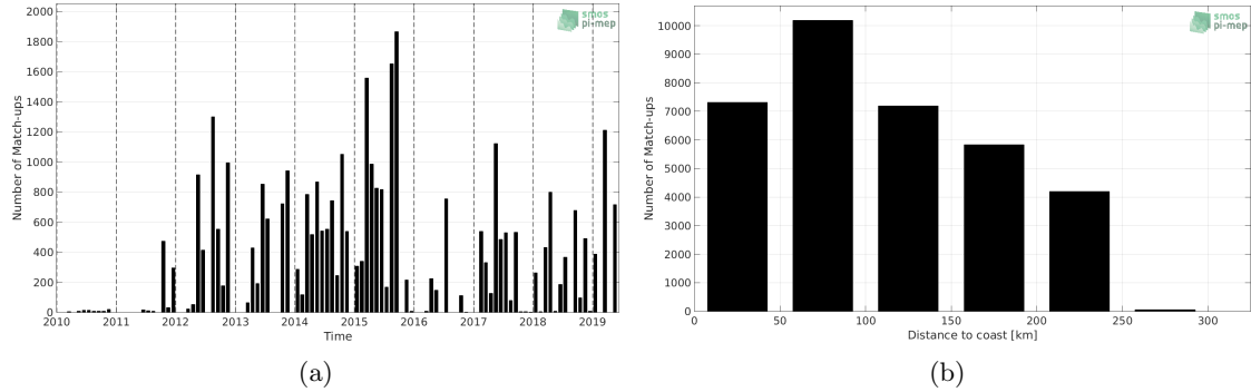
Figure 1: Number of match-ups between TSG-LEGOS-DM and SMOS L3 v317 - Monthly - 25 km (CATDS-CPDC) SSS as a function of time (a) and as function of the distance to coast (b) over the Sea of Japan Pi-MEP region and for the full satellite product period.
