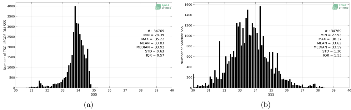
Figure 2: Histograms of SSS from TSG-LEGOS-DM (a) and SMOS L3 v317 - Monthly - 25 km (CATDS-CPDC) (b) considering all match-up pairs per bins of 0.1 over the Sea of Japan Pi-MEP region and for the full satellite product period.
