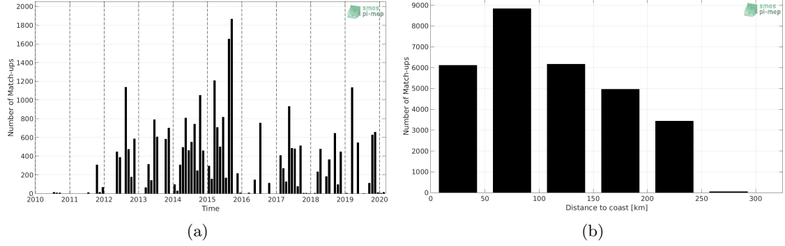
Figure 1: Number of match-ups between TSG (LEGOS-DM) and SMOS SSS L3 v317 - 10 Days - 25 km (CATDS-CPDC) SSS as a function of time (a) and as function of the distance to coast (b) over the Sea of Japan Pi-MEP region and for the full satellite product period.
