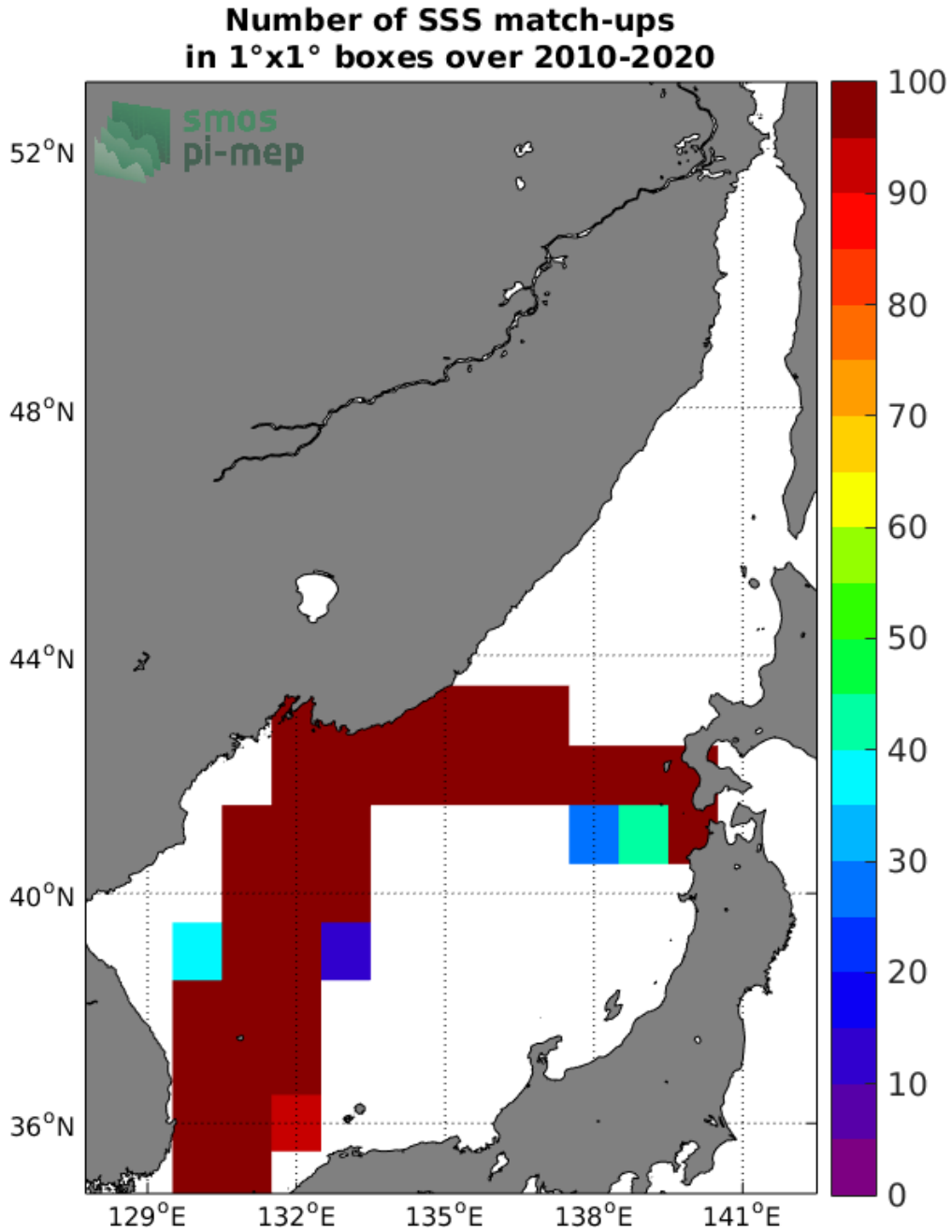
Figure 4: Number of SSS match-ups between TSG (LEGOS-DM) SSS and the SMOS SSS L3 v317 - 10 Days - 25 km (CATDS-CPDC) SSS product for the Sea of Japan Pi-MEP region over 1^\circ \times 1^\circ boxes and for the full satellite product period.
