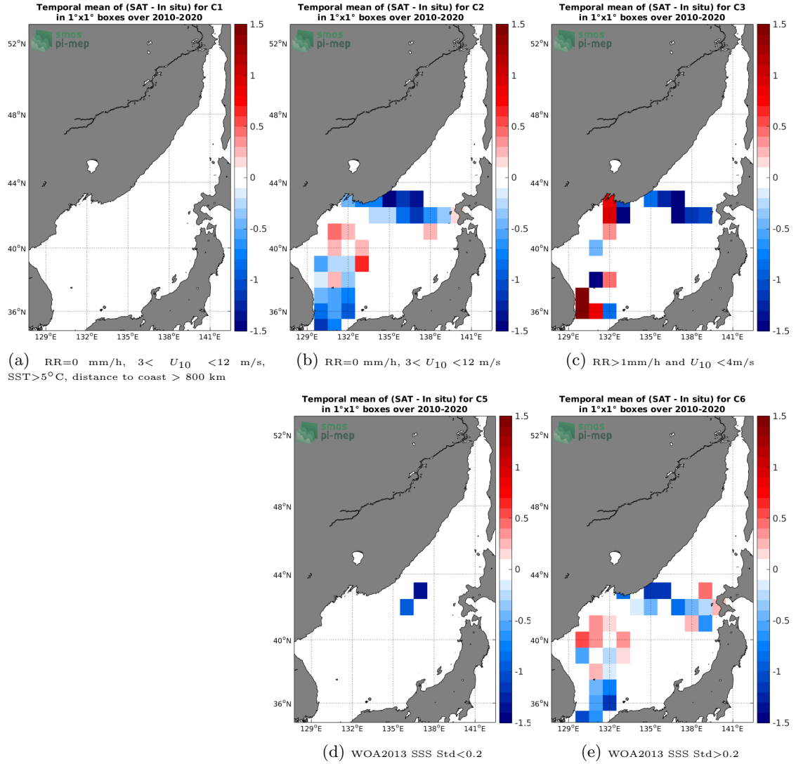
Figure 12: Temporal mean gridded over spatial boxes of size 1^\circ \times 1^\circ of \Delta\text{SSS} (SMOS SSS L3 v317 - 10 Days - 25 km (CATDS-CPDC) - TSG (LEGOS-DM)) for 5 different subdatasets corresponding to: RR=0 mm/h, 3 < U_{10} < 12 m/s, SST > 5^\circ\text{C} , distance to coast > 800 km (a), RR=0 mm/h, 3 < U_{10} < 12 m/s (b), RR > 1 mm/h and U_{10} < 4 m/s (c), WOA2013 SSS Std < 0.2 (d), WOA2013 SSS Std > 0.2 (e).
