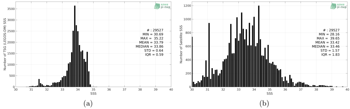
Figure 2: Histograms of SSS from TSG (LEGOS-DM) (a) and SMOS SSS L3 v317 - 10 Days - 25 km (CATDS-CPDC) (b) considering all match-up pairs per bins of 0.1 over the Sea of Japan Pi-MEP region and for the full satellite product period.
