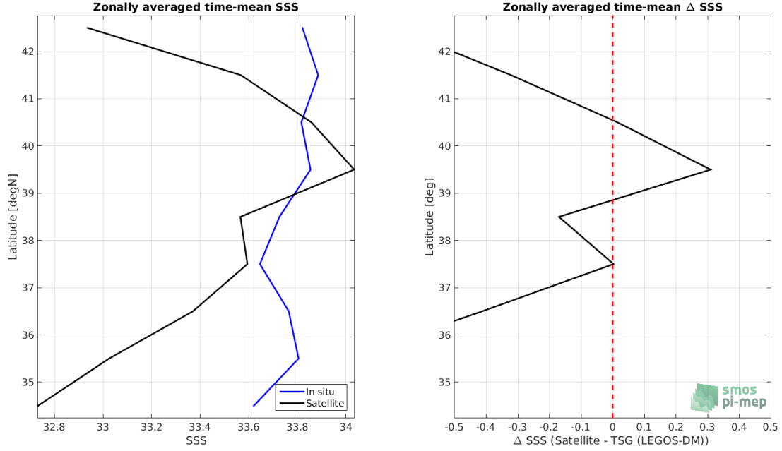
Figure 8: Left panel: Zonal mean SSS from SMOS SSS L3 v317 - 10 Days - 25 km (CATDS-CPDC) satellite product (black) and from TSG (LEGOS-DM) (blue). Right panel: Zonal mean of \Delta\text{SSS} (Satellite - TSG (LEGOS-DM)) for all the collected Pi-MEP match-up pairs estimated over the full satellite product period.
