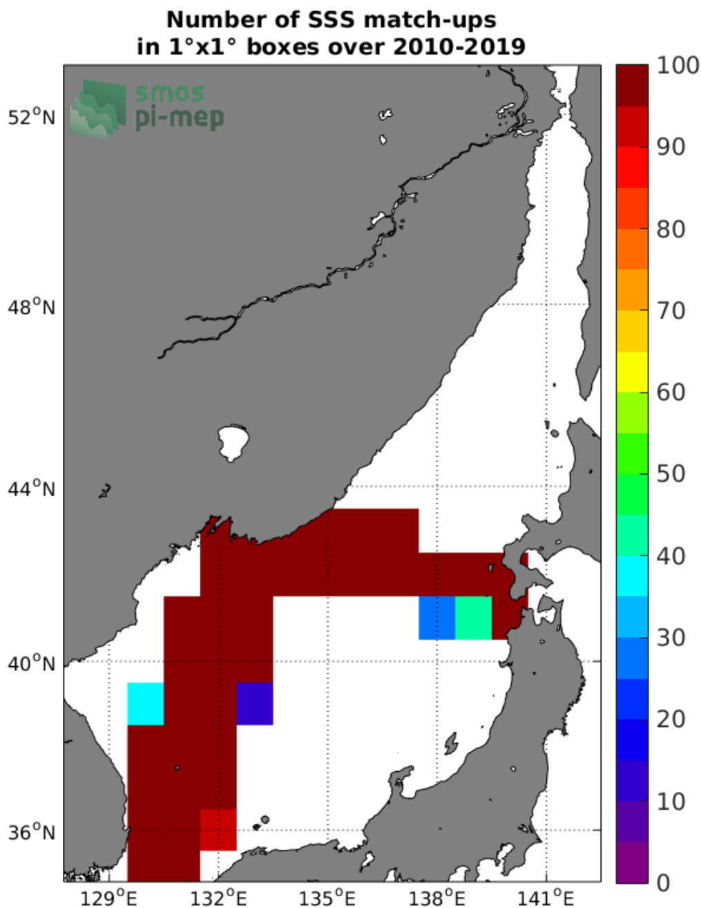
Figure 4: Number of SSS match-ups between TSG (LEGOS-DM) SSS and the SMOS SSS L3 v317 - 10 Days - 25 km (CATDS-CPDC) SSS product for the Sea of Japan Pi-MEP region over 1°x1° boxes and for the full satellite product period.
