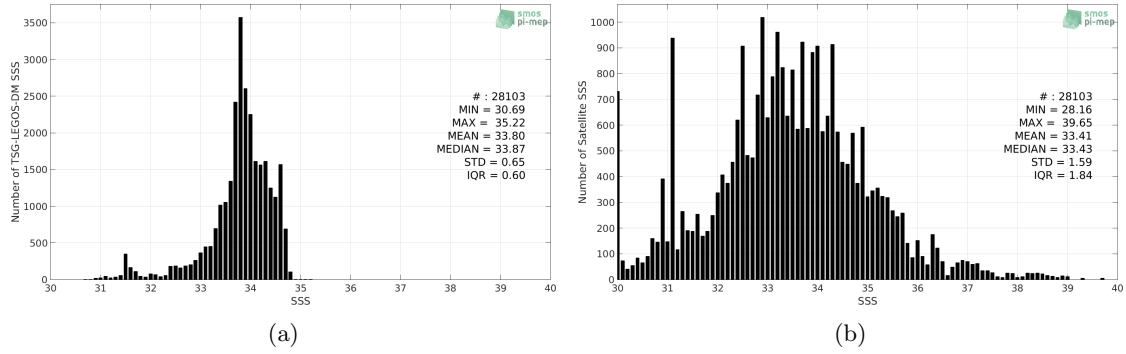
Figure 2: Histograms of SSS from TSG-LEGOS-DM (a) and SMOS L3 v317 - 10 Days - 25 km (CATDS-CPDC) (b) considering all match-up pairs per bins of 0.1 over the Sea of Japan Pi-MEP region and for the full satellite product period.
