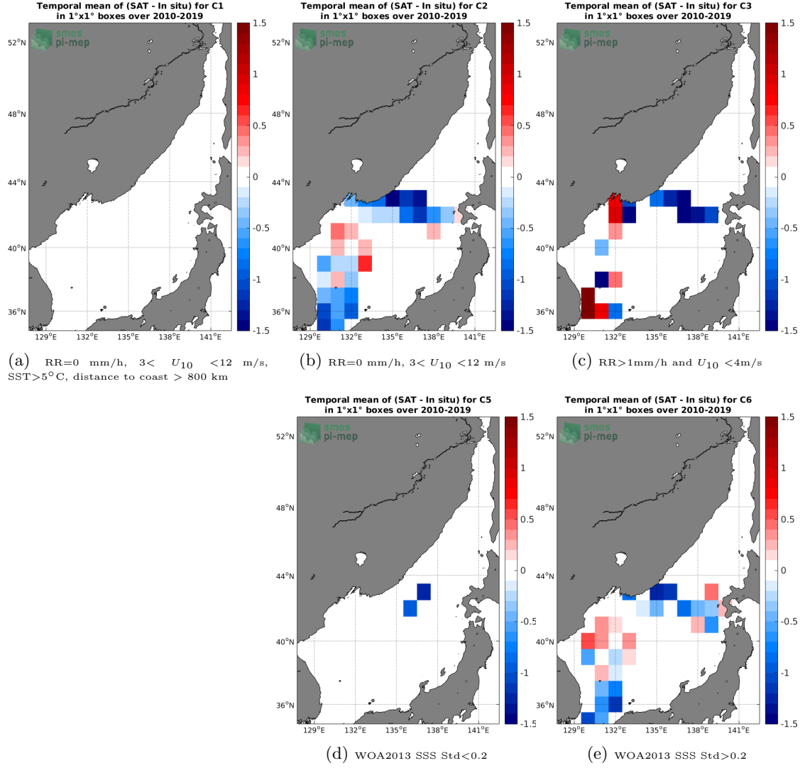
Figure 12: Temporal mean gridded over spatial boxes of size 1°x1° of \Delta\text{SSS} (SMOS L3 v317 - 10 Days - 25 km (CATDS-CPDC) - TSG-LEGOS-DM) for 5 different subdatasets corresponding to: RR=0 mm/h, 3 < U_{10} < 12 m/s, SST > 5^\circ\text{C} , distance to coast > 800 km (a), RR=0 mm/h, 3 < U_{10} < 12 m/s (b), RR > 1 mm/h and U_{10} < 4 m/s (c), WOA2013 SSS Std < 0.2 (d), WOA2013 SSS Std > 0.2 (e).
