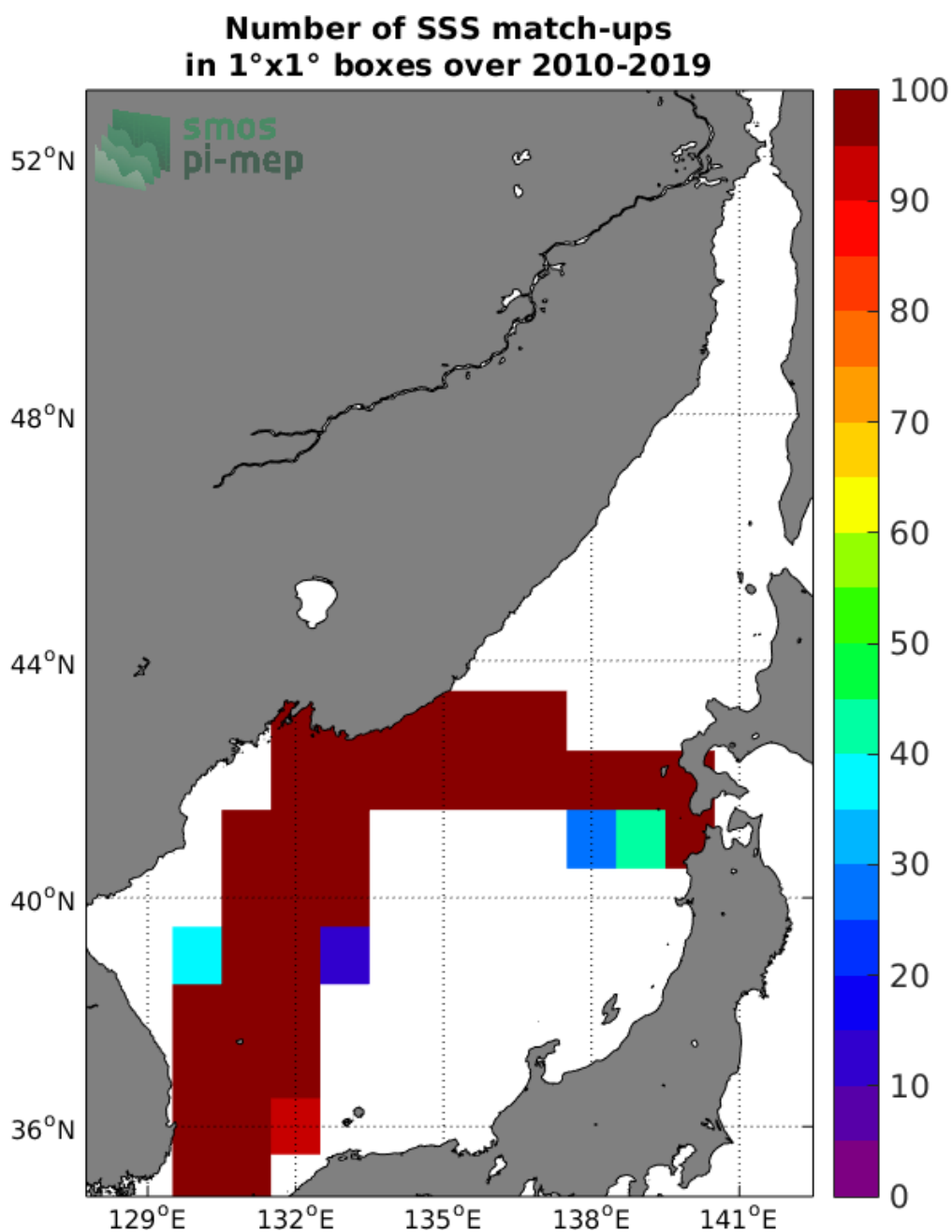
Figure 4: Number of SSS match-ups between TSG-LEGOS-DM SSS and the SMOS L3 v317 - 10 Days - 25 km (CATDS-CPDC) SSS product for the Sea of Japan Pi-MEP region over 1°x1° boxes and for the full satellite product period.
