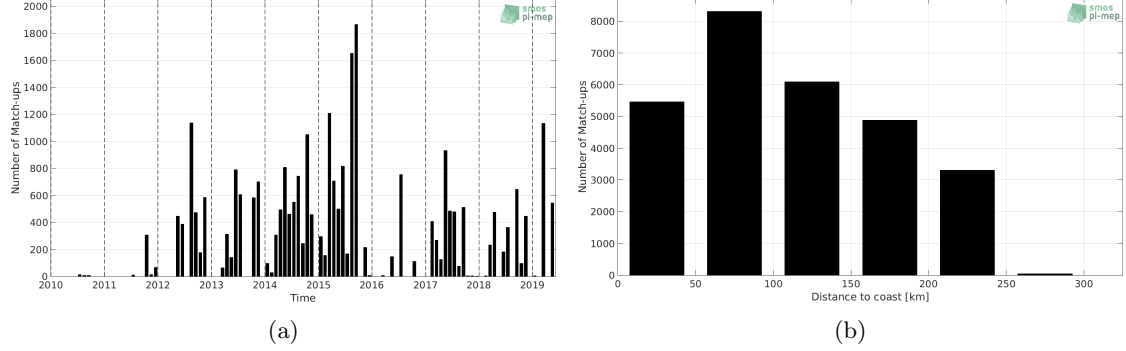
Figure 1: Number of match-ups between TSG-LEGOS-DM and SMOS L3 v317 - 10 Days - 25 km (CATDS-CPDC) SSS as a function of time (a) and as function of the distance to coast (b) over the Sea of Japan Pi-MEP region and for the full satellite product period.
