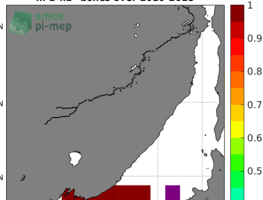
Temporal STD of (Sat - TSG-LEGOS-DM) in 1°x1° boxes over 2010-2018
