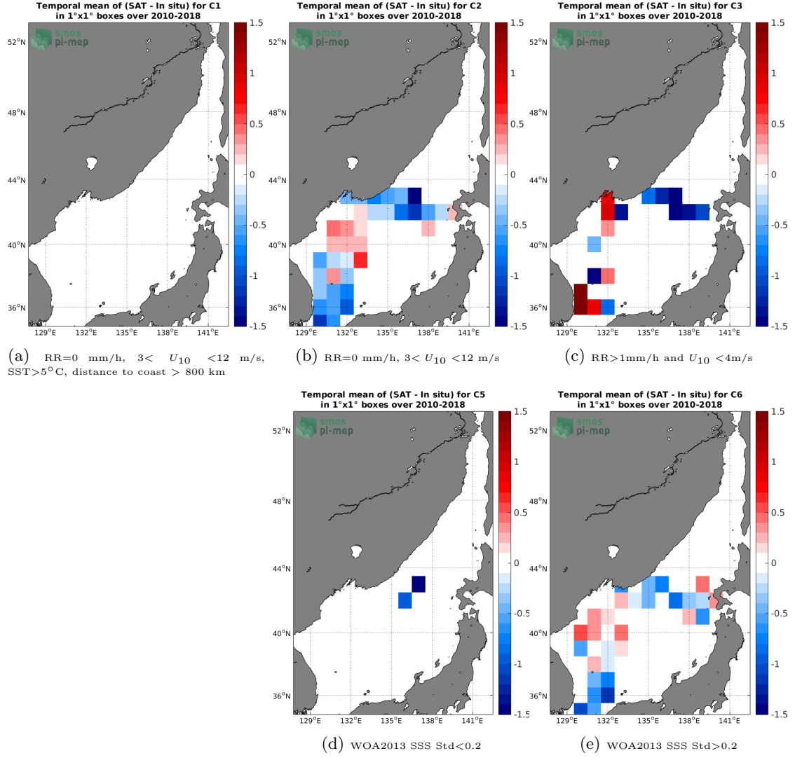
Figure 12: Temporal mean gridded over spatial boxes of size 1°x1° of \Delta\text{SSS} (SMOS-L3-CATDS-CPDC-V317-10DAYS-25KM - TSG-LEGOS-DM) for 5 different subdatasets corresponding to: RR=0 mm/h, 3 < U_{10} < 12 m/s, SST > 5^\circ\text{C} , distance to coast > 800 km (a), RR=0 mm/h, 3 < U_{10} < 12 m/s (b), RR > 1\text{mm/h} and U_{10} < 4\text{m/s} (c), WOA2013 SSS Std < 0.2 (d), WOA2013 SSS Std > 0.2 (e).
