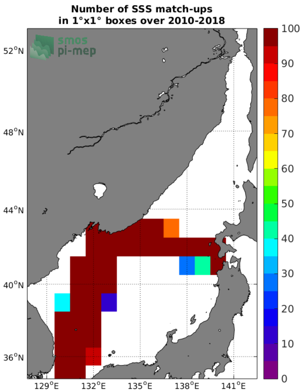
Figure 4: Number of SSS match-ups between TSG-LEGOS-DM SSS and the SMOS-L3-CATDS-CPDC-V317-10DAYS-25KM SSS product for the Sea of Japan Pi-MEP region over 1°x1° boxes and for the full satellite product period.
