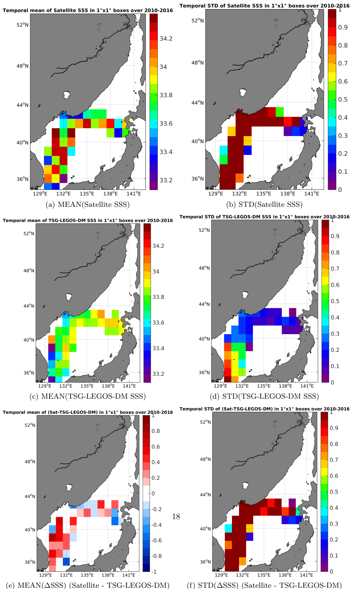
Figure 6: Temporal mean (left) and STD (right) of SSS from SMOS-L3-CATDS-CPDC-V3-MONTHLY-25KM (top), TSG-LEGOS-DM (middle), and of \Delta SSS (Satellite - TSG-LEGOS-DM). Only match-up pairs are used to generate these maps.
