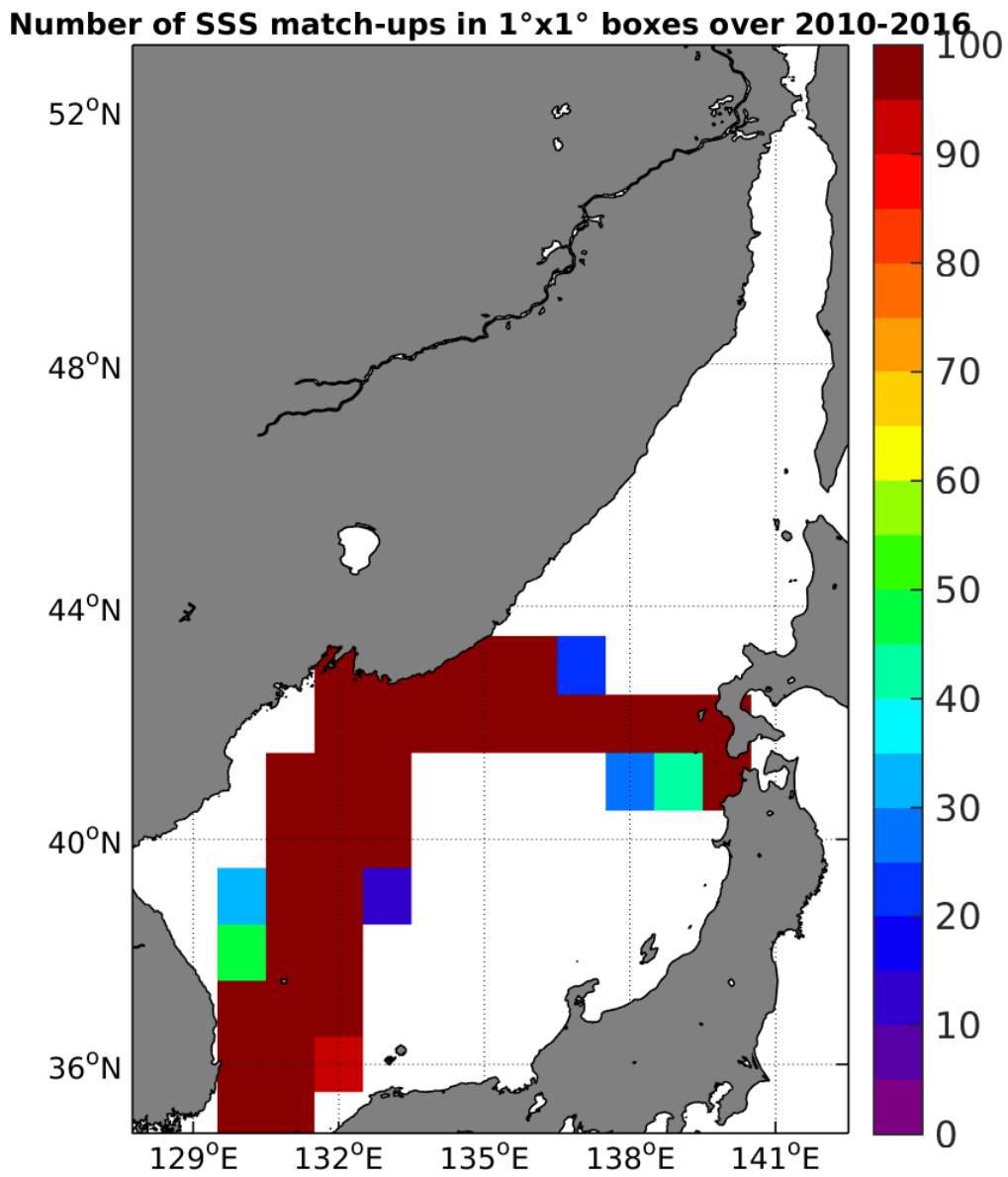
Figure 4: Number of SSS match-ups between TSG-LEGOS-DM SSS and the SMOS-L3-CATDS-CPDC-V3-MONTHLY-25KM SSS product for the Sea of Japan Pi-MEP region over 1°x1° boxes and for the full satellite product period.
