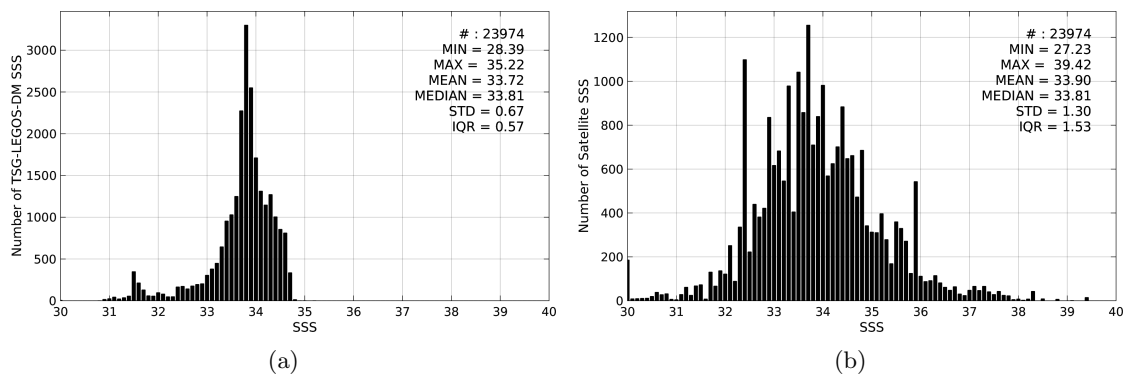
Figure 2: Histograms of SSS from TSG-LEGOS-DM (a) and SMOS-L3-CATDS-CPDC-V3-MONTHLY-25KM (b) considering all match-up pairs per bins of 0.1 over the Sea of Japan Pi-MEP region and for the full satellite product period.
