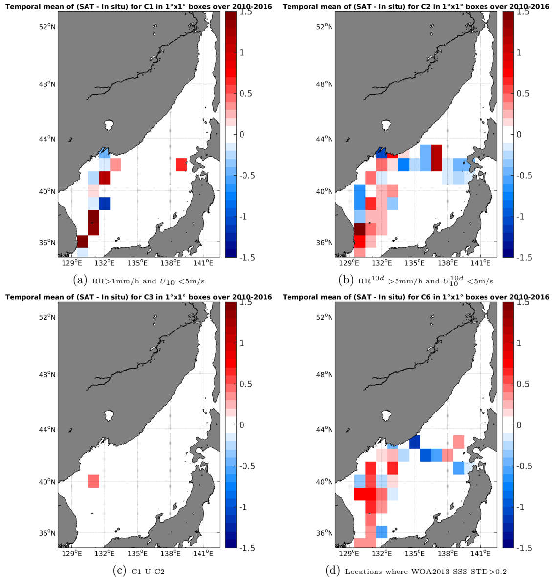
Figure 12: Temporal mean gridded over spatial boxes of size 1^\circ \times 1^\circ of \Delta SSS (SMOS-L3-CATDS-CPDC-V3-MONTHLY-25KM - TSG-LEGOS-DM) for 4 different subdatasets corresponding to: RR > 1\text{mm/h} and U_{10} < 5\text{m/s} (a), RR^{10d} > 5\text{mm/h} and U_{10}^{10d} < 5\text{m/s} (b), C1 U C2 (c), Locations where WOA2013 SSS STD > 0.2 (d).
