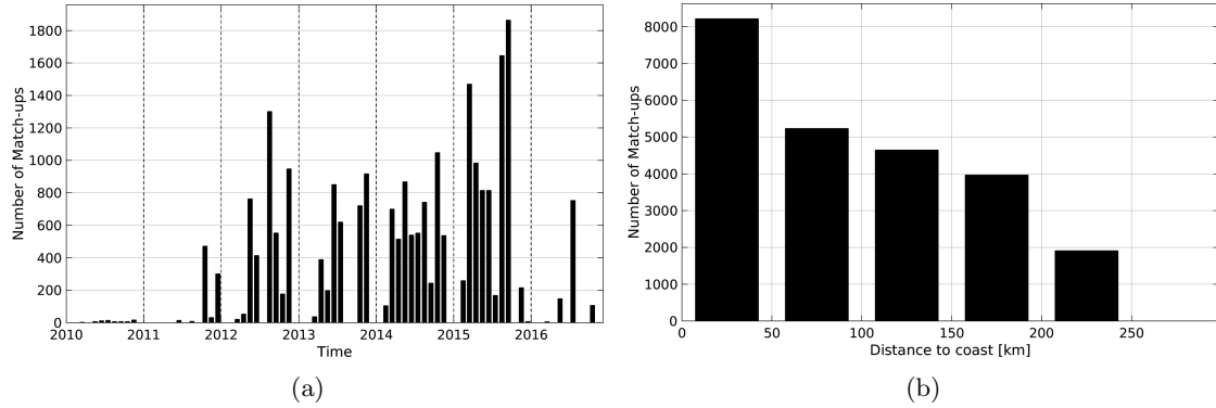
Figure 1: Number of match-ups between TSG-LEGOS-DM and SMOS-L3-CATDS-CPDC-V3-MONTHLY-25KM SSS as a function of time (a) and as function of the distance to coast (b) over the Sea of Japan Pi-MEP region and for the full satellite product period.
