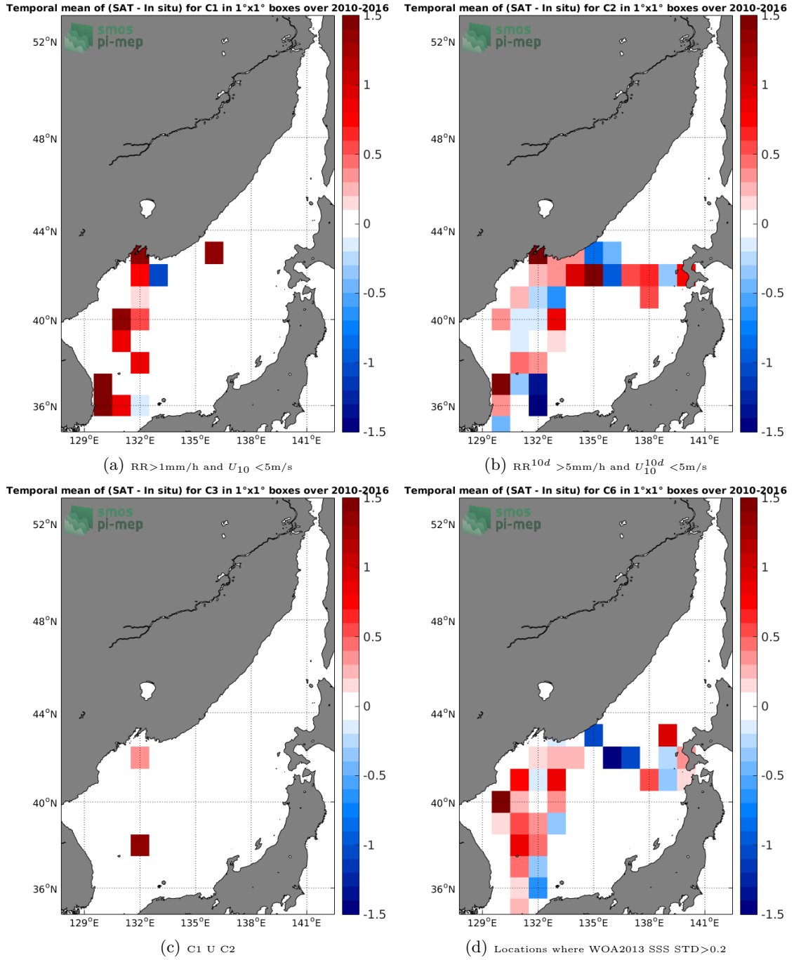
Figure 12: Temporal mean gridded over spatial boxes of size 1°x1° of \Delta\text{SSS} (SMOS-L3-CATDS-CPDC-V3-10DAYS-25KM - TSG-LEGOS-DM) for 4 different subdatasets corresponding to: RR > 1\text{mm/h} and U_{10} < 5\text{m/s} (a), RR^{10d} > 5\text{mm/h} and U_{10}^{10d} < 5\text{m/s} (b), C1 U C2 (c), Locations where WOA2013 SSS STD > 0.2 (d).
