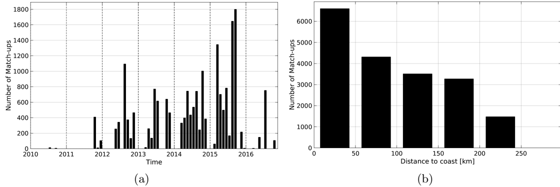
Figure 1: Number of match-ups between TSG-LEGOS-DM and SMOS-L3-CATDS-CPDC-V3-10DAYS-25KM SSS as a function of time (a) and as function of the distance to coast (b) over the Sea of Japan Pi-MEP region and for the full satellite product period.
