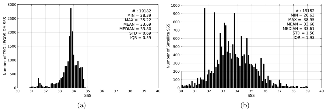
Figure 2: Histograms of SSS from TSG-LEGOS-DM (a) and SMOS-L3-CATDS-CPDC-V3-10DAYS-25KM (b) considering all match-up pairs per bins of 0.1 over the Sea of Japan Pi-MEP region and for the full satellite product period.
