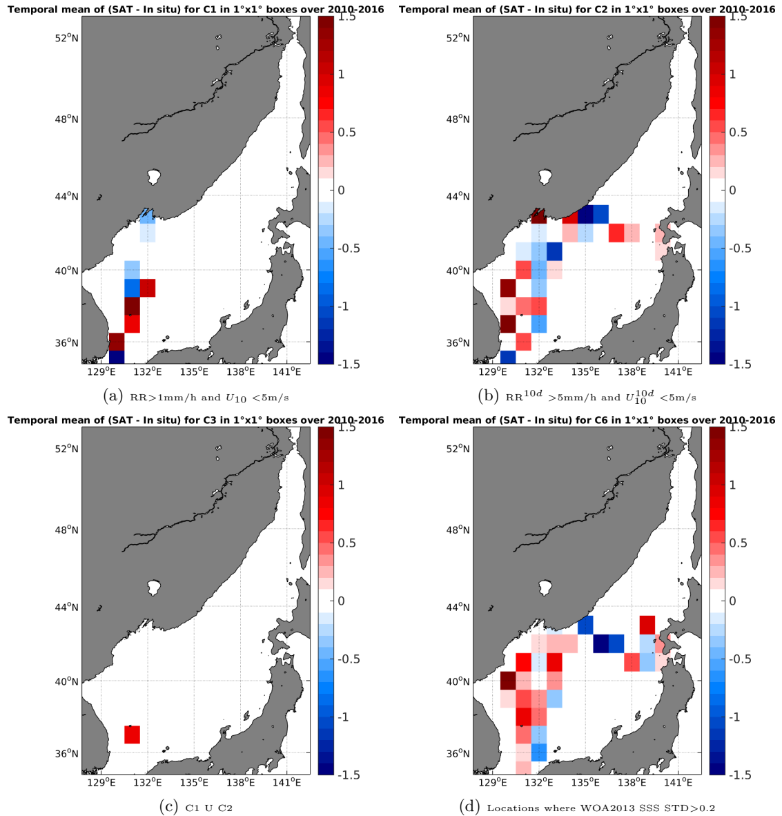
Figure 12: Temporal mean gridded over spatial boxes of size 1^\circ \times 1^\circ of \Delta SSS (SMOS-L3-CATDS-CPDC-V3-10DAYS-25KM - TSG-LEGOS-DM) for 4 different subdatasets corresponding to: RR > 1\text{mm/h} and U_{10} < 5\text{m/s} (a), RR^{10d} > 5\text{mm/h} and U_{10}^{10d} < 5\text{m/s} (b), C1 U C2 (c), Locations where WOA2013 SSS STD > 0.2 (d).
