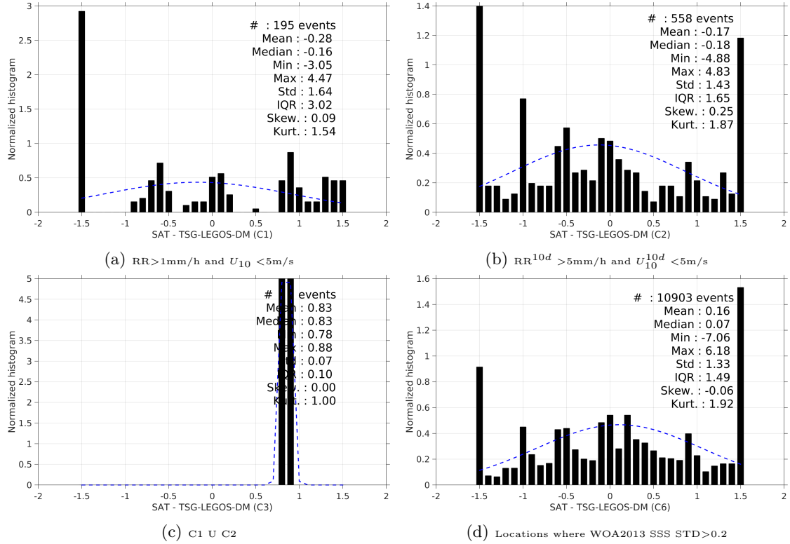
Figure 13: Normalized histogram of \Delta\text{SSS} (SMOS-L3-CATDS-CPDC-V3-10DAYS-25KM - TSG-LEGOS-DM) for 6 different subdatasets corresponding to: RR > 1mm/h and U_{10} < 5\text{m/s} (a), \text{RR}^{10d} > 5\text{mm/h} and U_{10}^{10d} < 5\text{m/s} (b), C1 U C2 (c), Locations where WOA2013 SSS STD > 0.2 (d).
