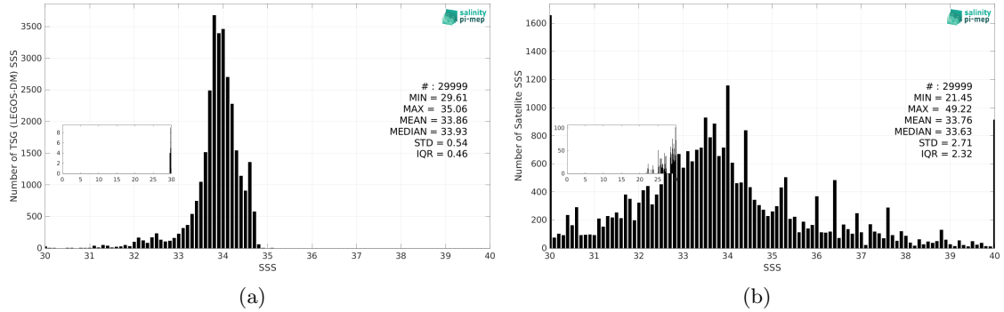
Figure 3: Histograms of SSS from TSG (LEGOS-DM) (a) and SMOS SSS L3 v2 - 9-Days (BEC) (b) considering all match-up pairs per bins of 0.1 over the Sea of Japan Pi-MEP region and for the full satellite product period.
