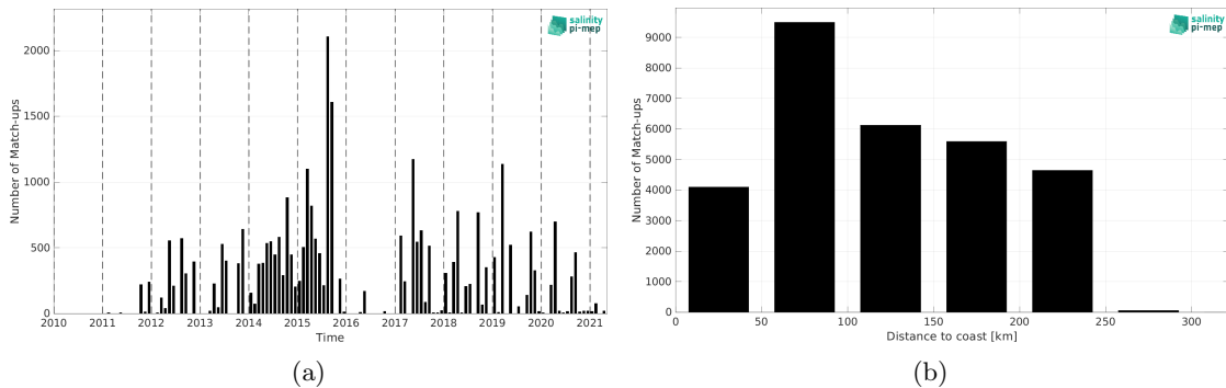
Figure 2: Number of match-ups between TSG (LEGOS-DM) and SMOS SSS L3 v2 - 9-Days (BEC) SSS as a function of time (a) and as function of the distance to coast (b) over the Sea of Japan Pi-MEP region and for the full satellite product period.
