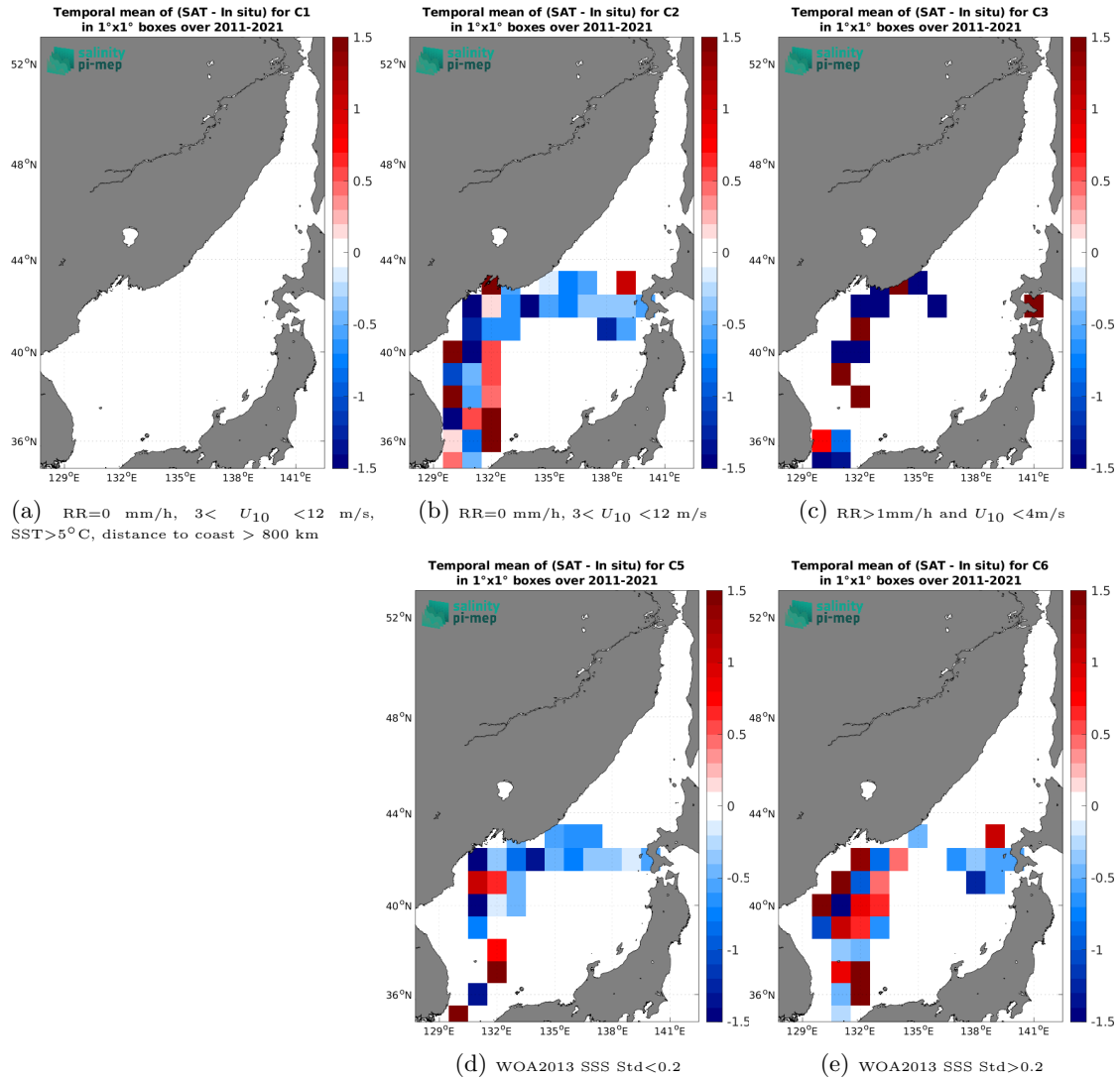
Figure 14: Temporal mean gridded over spatial boxes of size 1^\circ \times 1^\circ of \Delta\text{SSS} (SMOS SSS L3 v2 - 9-Days (BEC) - TSG (LEGOS-DM)) for 5 different subdatasets corresponding to: RR=0 mm/h, 3 < U_{10} < 12 m/s, SST > 5^\circ\text{C} , distance to coast > 800 km (a), RR=0 mm/h, 3 < U_{10} < 12 m/s (b), RR > 1 mm/h and U_{10} < 4 m/s (c), WOA2013 SSS Std < 0.2 (d), WOA2013 SSS Std > 0.2 (e).
