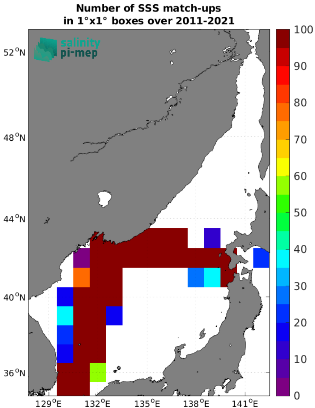
Figure 5: Number of SSS match-ups between TSG (LEGOS-DM) SSS and the SMOS SSS L3 v2 - 9-Days (BEC) SSS product for the Sea of Japan Pi-MEP region over 1°x1° boxes and for the full satellite product period.
