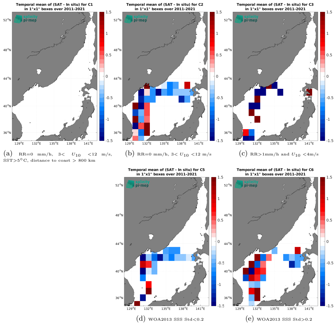
Figure 14: Temporal mean gridded over spatial boxes of size 1^\circ \times 1^\circ of \Delta SSS (SMOS SSS L3 v2 - 9-Days (BEC) - TSG (LEGOS-DM)) for 5 different subdatasets corresponding to: RR=0 mm/h, 3 < U_{10} < 12 m/s, SST > 5^\circ C , distance to coast > 800 km (a), RR=0 mm/h, 3 < U_{10} < 12 m/s (b), RR > 1 mm/h and U_{10} < 4 m/s (c), WOA2013 SSS Std < 0.2 (d), WOA2013 SSS Std > 0.2 (e).
