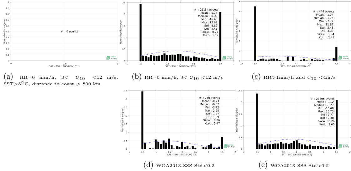
Figure 13: Normalized histogram of \Delta\text{SSS} (SMOS SSS L3 v2 - 9-Days (BEC) - TSG (LEGOS-DM)) for 5 different subdatasets corresponding to: RR=0 mm/h, 3 < U_{10} < 12 m/s, SST > 5^{\circ}\text{C} , distance to coast > 800 km (a), RR=0 mm/h, 3 < U_{10} < 12 m/s (b), RR > 1\text{mm/h} and U_{10} < 4\text{m/s} (c), WOA2013 SSS Std < 0.2 (d), WOA2013 SSS Std > 0.2 (e).
