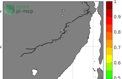
Temporal STD of (Sat - TSG (LEGOS-DM)) in 1°x1° boxes over 2011-2019
