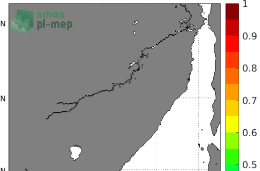
Temporal STD of (Sat - TSG (LEGOS-DM)) in 1°x1° boxes over 2011-2019
