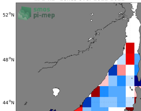
Temporal mean of (Sat - Argo) in 1°x1° boxes over 2011-2021
