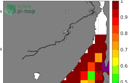
Temporal STD of (Sat - Argo) in 1°x1° boxes over 2011-2019
