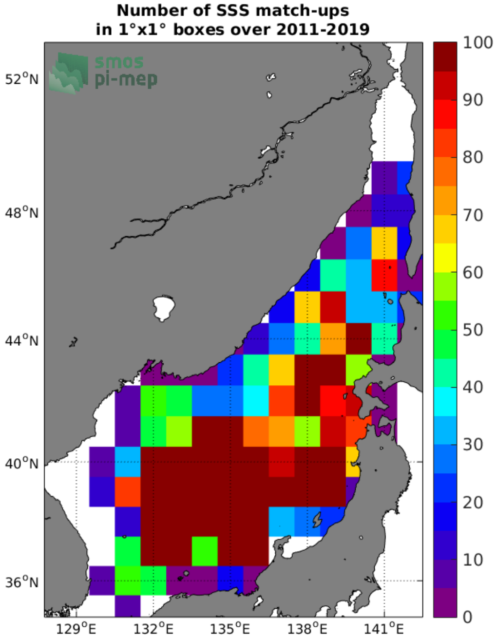
Figure 4: Number of SSS match-ups between Argo SSS and the SMOS SSS L3 v2 - 9-Days (BEC) SSS product for the Sea of Japan Pi-MEP region over 1^\circ \times 1^\circ boxes and for the full satellite product period.
