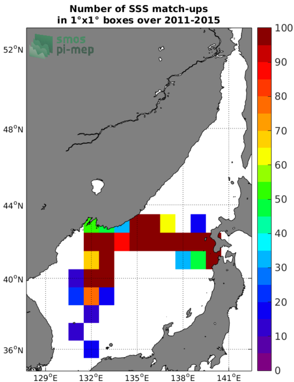
Figure 4: Number of SSS match-ups between TSG-LEGOS-DM SSS and the SMOS-L3-BEC-OA-V1-9DAYS-0.25DEG SSS product for the Sea of Japan Pi-MEP region over 1°x1° boxes and for the full satellite product period.
