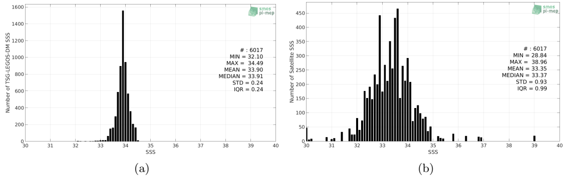
Figure 2: Histograms of SSS from TSG-LEGOS-DM (a) and SMOS-L3-BEC-OA-V1-9DAYS-0.25DEG (b) considering all match-up pairs per bins of 0.1 over the Sea of Japan Pi-MEP region and for the full satellite product period.
