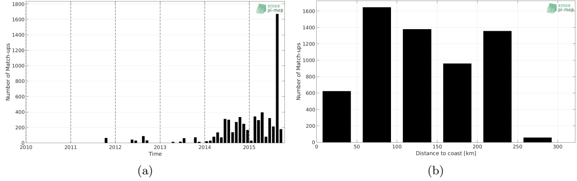
Figure 1: Number of match-ups between TSG-LEGOS-DM and SMOS-L3-BEC-OA-V1-9DAYS-0.25DEG SSS as a function of time (a) and as function of the distance to coast (b) over the Sea of Japan Pi-MEP region and for the full satellite product period.
