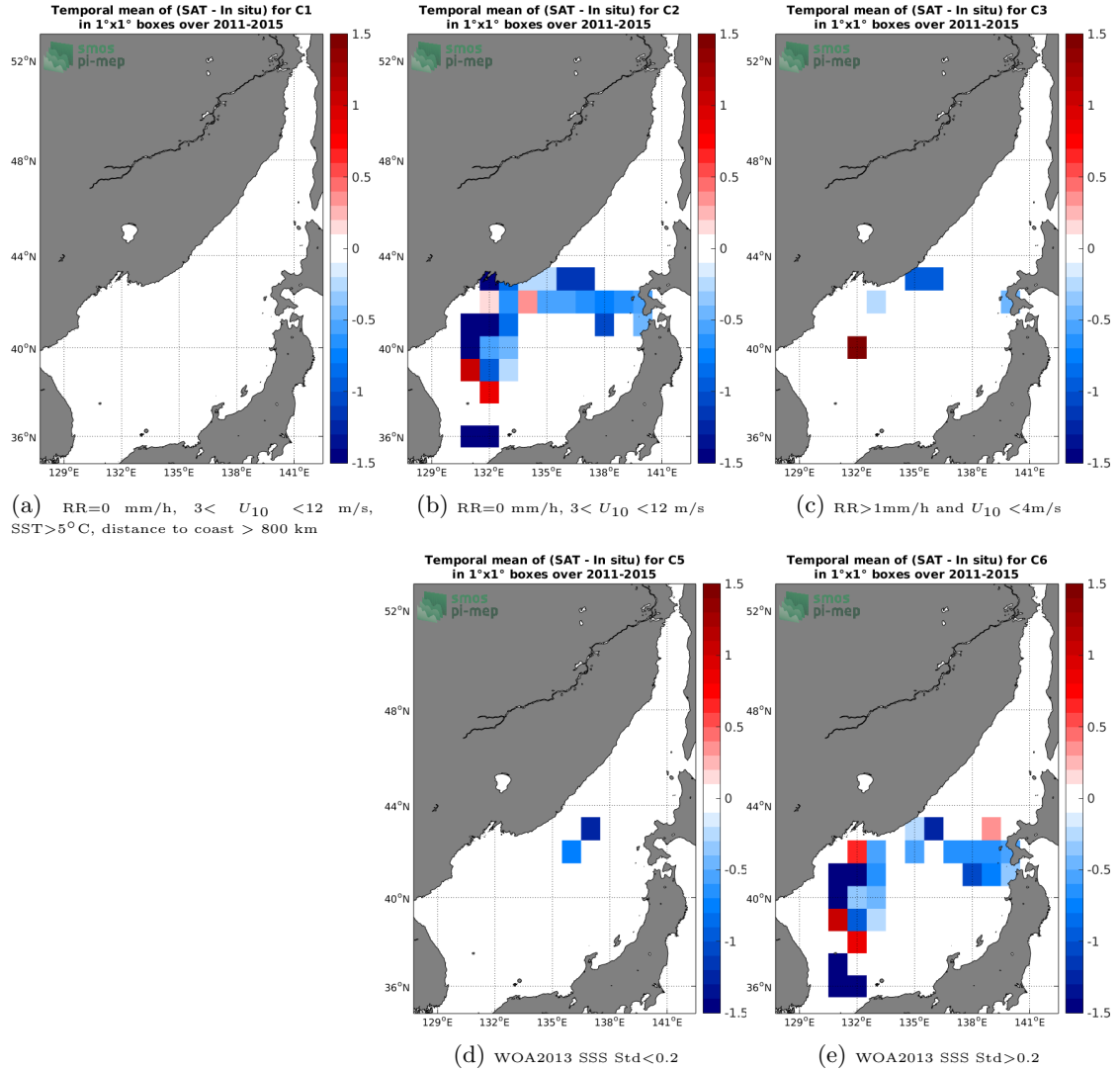
Figure 12: Temporal mean gridded over spatial boxes of size 1°x1° of \Delta\text{SSS} (SMOS-L3-BEC-OA-V1-9DAYS-0.25DEG - TSG-LEGOS-DM) for 5 different subdatasets corresponding to: RR=0 mm/h, 3 < U_{10} < 12 m/s, SST > 5^\circ\text{C} , distance to coast > 800 km (a), RR=0 mm/h, 3 < U_{10} < 12 m/s (b), RR > 1 mm/h and U_{10} < 4 m/s (c), WOA2013 SSS Std < 0.2 (d), WOA2013 SSS Std > 0.2 (e).
