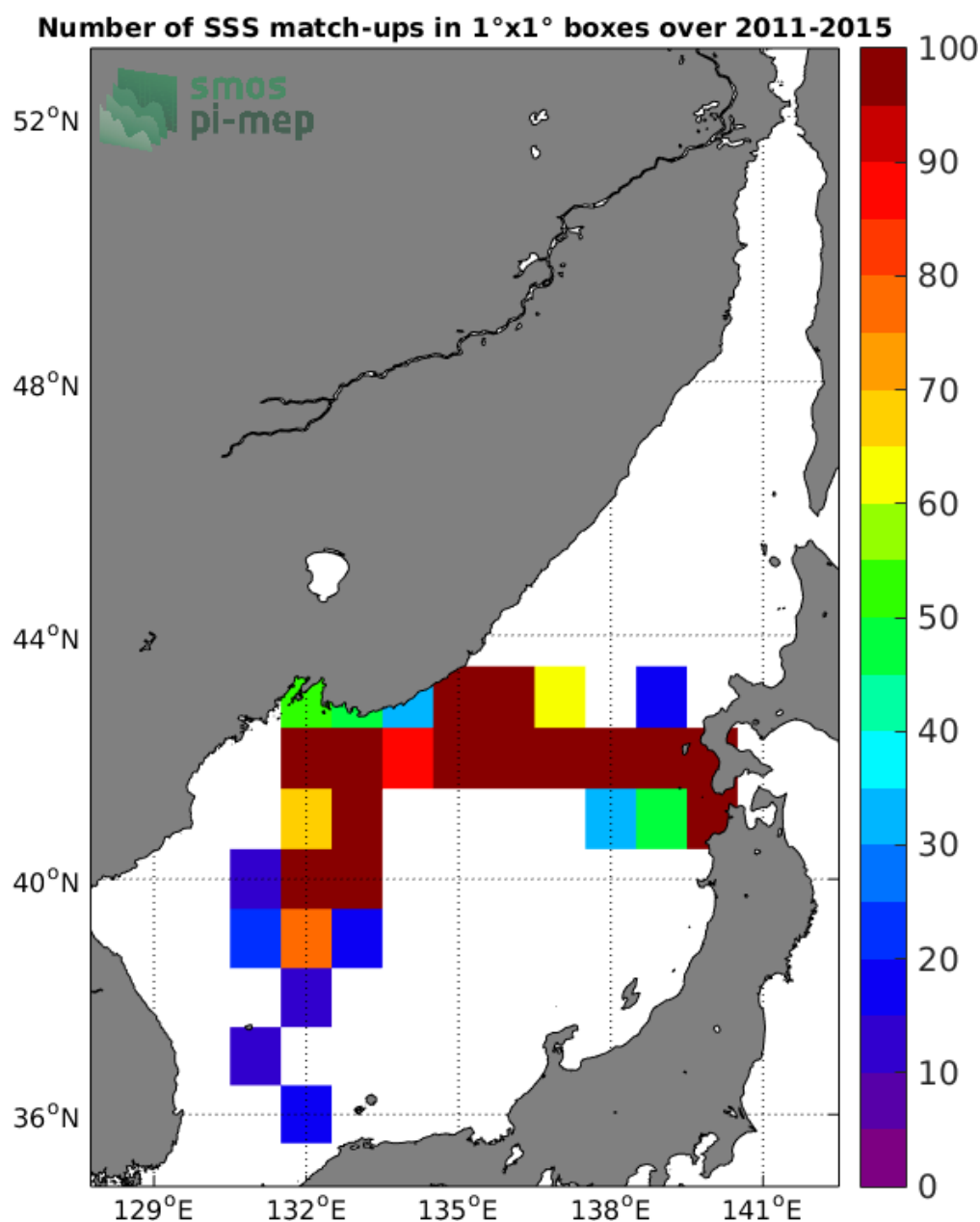
Figure 4: Number of SSS match-ups between TSG-LEGOS-DM SSS and the SMOS-L3-BEC-OA-V1-9DAYS-0.25DEG SSS product for the Sea of Japan Pi-MEP region over 1°x1° boxes and for the full satellite product period.
