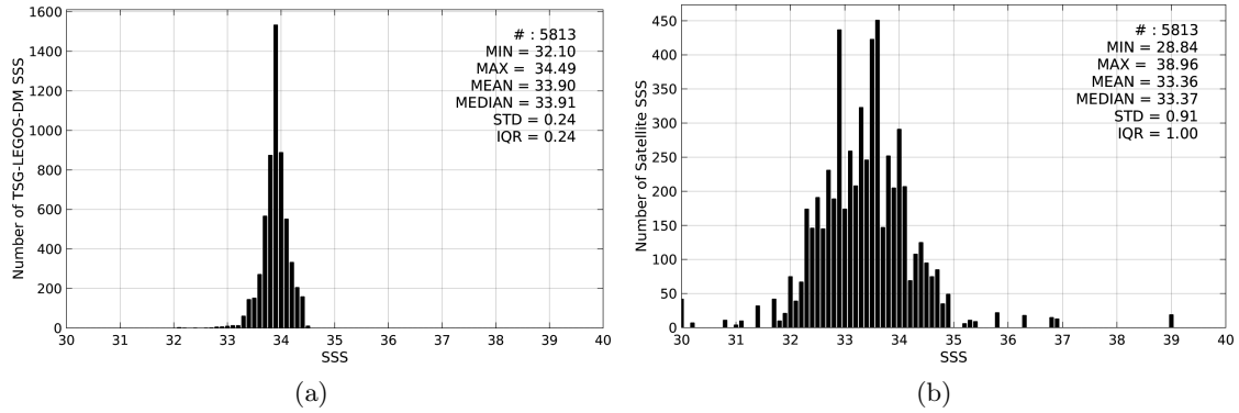
Figure 2: Histograms of SSS from TSG-LEGOS-DM (a) and SMOS-L3-BEC-OA-V1-9DAYS-0.25DEG (b) considering all match-up pairs per bins of 0.1 over the Sea of Japan Pi-MEP region and for the full satellite product period.
