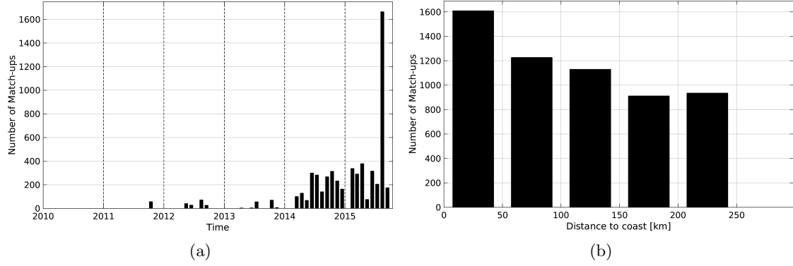
Figure 1: Number of match-ups between TSG-LEGOS-DM and SMOS-L3-BEC-OA-V1-9DAYS-0.25DEG SSS as a function of time (a) and as function of the distance to coast (b) over the Sea of Japan Pi-MEP region and for the full satellite product period.
