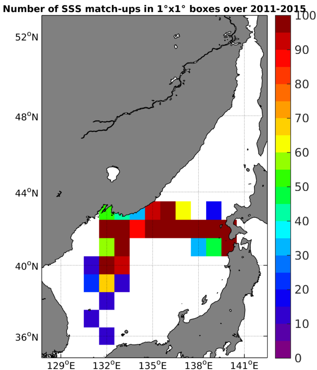
Figure 4: Number of SSS match-ups between TSG-LEGOS-DM SSS and the SMOS-L3-BEC-OA-V1-9DAYS-0.25DEG SSS product for the Sea of Japan Pi-MEP region over 1°x1° boxes and for the full satellite product period.
