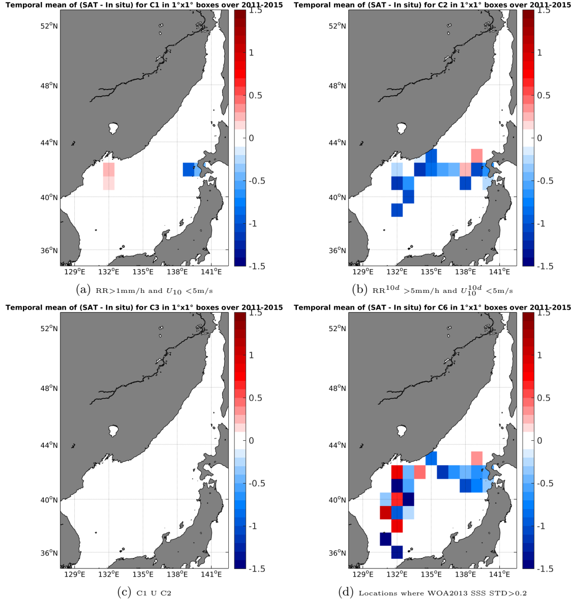
Figure 12: Temporal mean gridded over spatial boxes of size 1^\circ \times 1^\circ of \Delta SSS (SMOS-L3-BEC-OA-V1-9DAYS-0.25DEG - TSG-LEGOS-DM) for 4 different subdatasets corresponding to: RR > 1 mm/h and U_{10} < 5 m/s (a), RR 10d > 5 mm/h and U_{10}^{10d} < 5 m/s (b), C1 U C2 (c), Locations where WOA2013 SSS STD > 0.2 (d).
