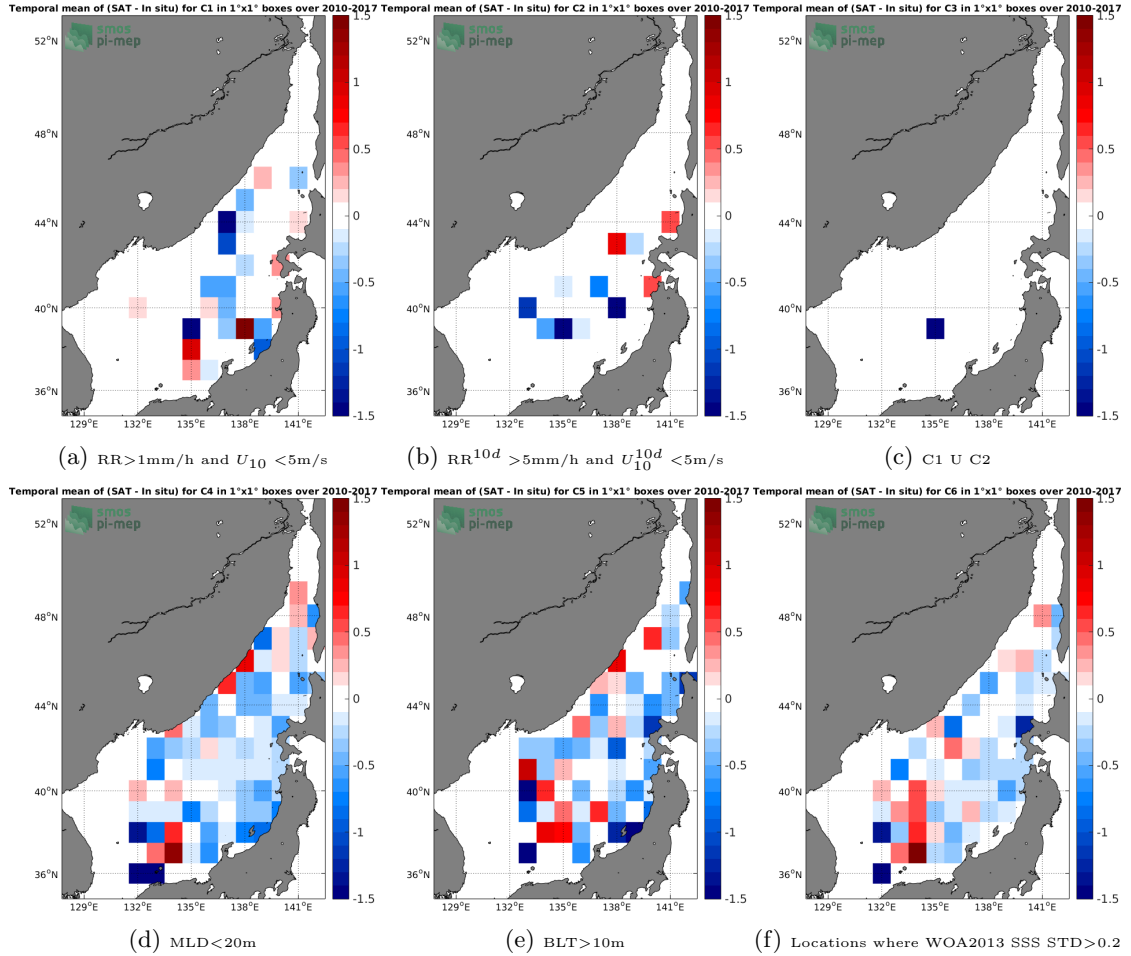
Figure 12: Temporal mean gridded over spatial boxes of size 1°x1° of \Delta SSS (SMOS-L3-BEC-OA-V1-9DAYS-0.25DEG - Argo) for 6 different subdatasets corresponding to:RR>1mm/h and U_{10} < 5\text{m/s} (a), RR^{10d} > 5\text{mm/h} and U_{10}^{10d} < 5\text{m/s} (b), C1 U C2 (c),MLD<20m (d),BLT>10m (e),Locations where WOA2013 SSS STD>0.2 (f).
