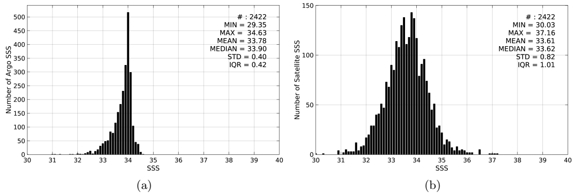
Figure 2: Histograms of SSS from Argo (a) and SMOS-L3-BEC-OA-V1-9DAYS-0.25DEG (b) considering all match-up pairs per bins of 0.1 over the Sea of Japan Pi-MEP region and for the full satellite product period.
