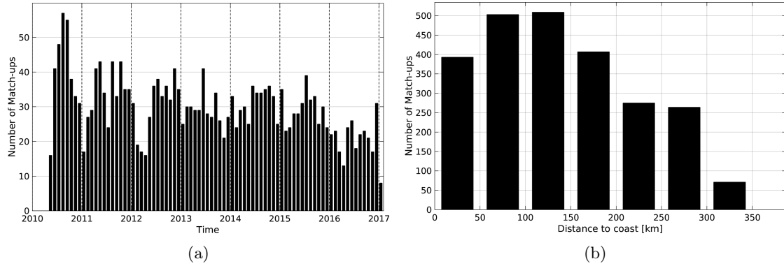
Figure 1: Number of match-ups between Argo and SMOS-L3-BEC-OA-V1-9DAYS-0.25DEG SSS as a function of time (a) and as function of the distance to coast (b) over the Sea of Japan Pi-MEP region and for the full satellite product period.
