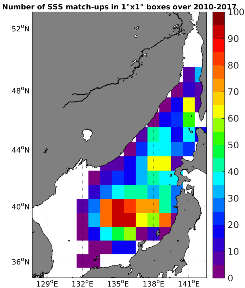
Figure 4: Number of SSS match-ups between Argo SSS and the SMOS-L3-BEC-OA-V1-9DAYS-0.25DEG SSS product for the Sea of Japan Pi-MEP region over 1°x1° boxes and for the full satellite product period.
