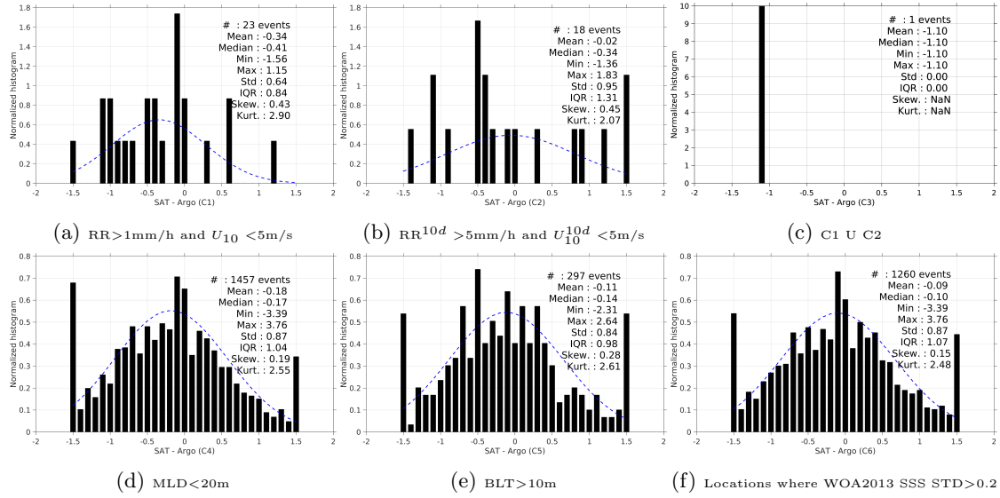
Figure 13: Normalized histogram of \Delta SSS (SMOS-L3-BEC-OA-V1-9DAYS-0.25DEG - Argo) for 6 different subdatasets corresponding to: RR>1mm/h and U_{10} < 5\text{m/s} (a), RR^{10d} > 5\text{mm/h} and U_{10}^{10d} < 5\text{m/s} (b), C1 U C2 (c),MLD<20m (d),BLT>10m (e),Locations where WOA2013 SSS STD>0.2 (f).
