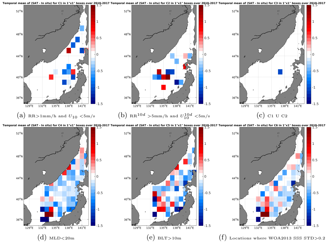
Figure 12: Temporal mean gridded over spatial boxes of size 1°x1° of \Delta SSS (SMOS-L3-BEC-OA-V1-9DAYS-0.25DEG - Argo) for 6 different subdatasets corresponding to:RR>1mm/h and U_{10} < 5\text{m/s} (a), RR^{10d} > 5\text{mm/h} and U_{10}^{10d} < 5\text{m/s} (b), C1 U C2 (c),MLD<20m (d),BLT>10m (e),Locations where WOA2013 SSS STD>0.2 (f).
