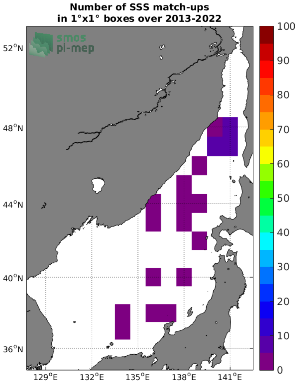
Figure 4: Number of SSS match-ups between Argo SSS and the SMOS SSS L2-AVERAGED v700 (ESA) SSS product for the Sea of Japan Pi-MEP region over 1°x1° boxes and for the full satellite product period.
