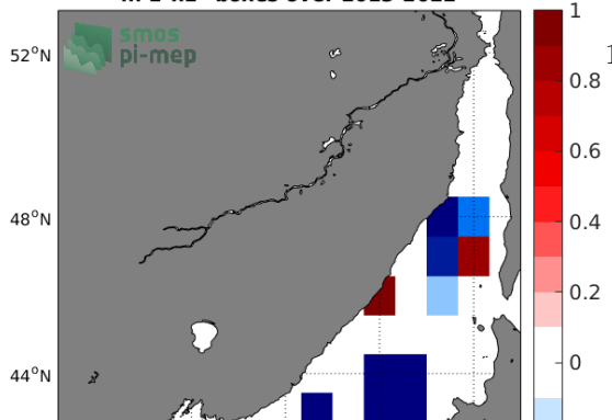
Temporal mean of (Sat - Argo) in 1°x1° boxes over 2013-2022
