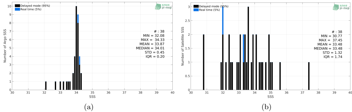
Figure 2: Histograms of SSS from Argo (a) and SMOS SSS L2-AVERAGED v700 (ESA) (b) considering all match-up pairs per bins of 0.1 over the Sea of Japan Pi-MEP region and for the full satellite product period.
