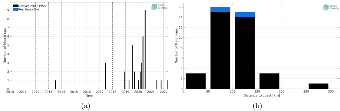
Figure 1: Number of match-ups between Argo and SMOS SSS L2-AVERAGED v700 (ESA) SSS as a function of time (a) and as function of the distance to coast (b) over the Sea of Japan Pi-MEP region and for the full satellite product period.
