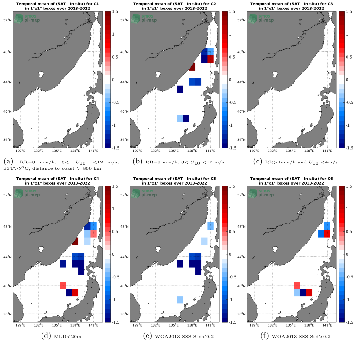
Figure 12: Temporal mean gridded over spatial boxes of size 1^\circ \times 1^\circ of \Delta\text{SSS} (SMOS SSS L2-AVERAGED v700 (ESA) - Argo) for 6 different subdatasets corresponding to: RR=0 mm/h, 3 < U_{10} < 12 m/s, SST > 5^\circ\text{C} , distance to coast > 800 km (a), RR=0 mm/h, 3 < U_{10} < 12 m/s (b), RR > 1 mm/h and U_{10} < 4 m/s (c), MLD < 20 m (d), WOA2013 SSS Std < 0.2 (e), WOA2013 SSS Std > 0.2 (f).
