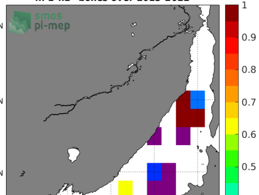
Temporal STD of (Sat - Argo) in 1°x1° boxes over 2013-2022
