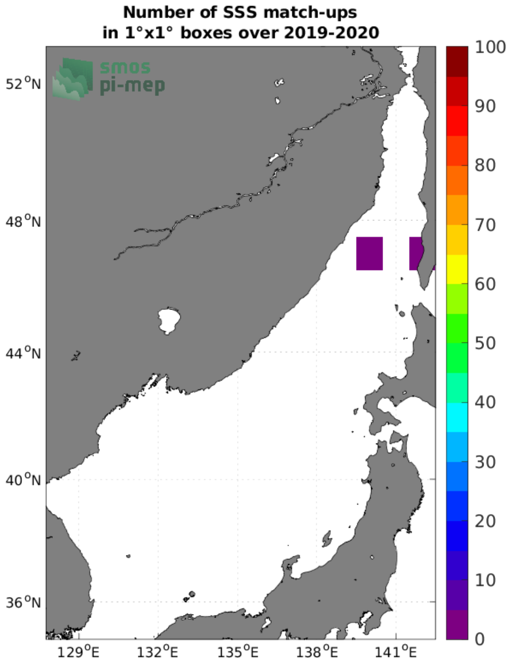
Figure 4: Number of SSS match-ups between Argo SSS and the SMOS SSS L2 v700 (ESA) SSS product for the Sea of Japan Pi-MEP region over 1°x1° boxes and for the full satellite product period.
