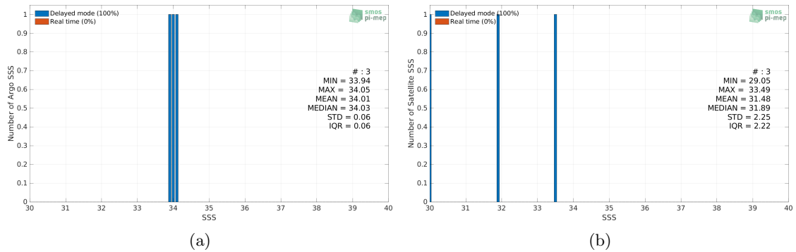
Figure 2: Histograms of SSS from Argo (a) and SMOS SSS L2 v700 (ESA) (b) considering all match-up pairs per bins of 0.1 over the Sea of Japan Pi-MEP region and for the full satellite product period.
