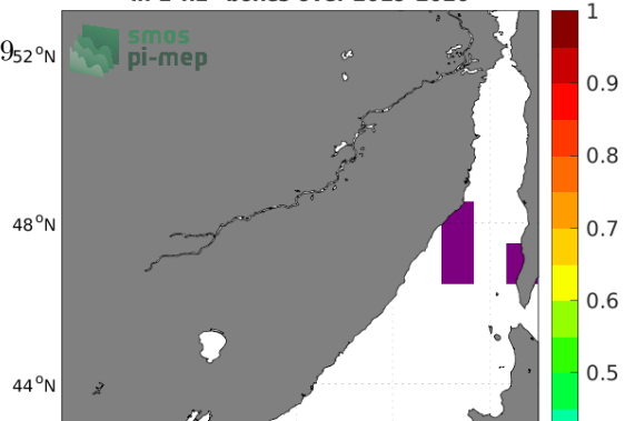
Temporal STD of (Sat - Argo) in 1°x1° boxes over 2019-2020
