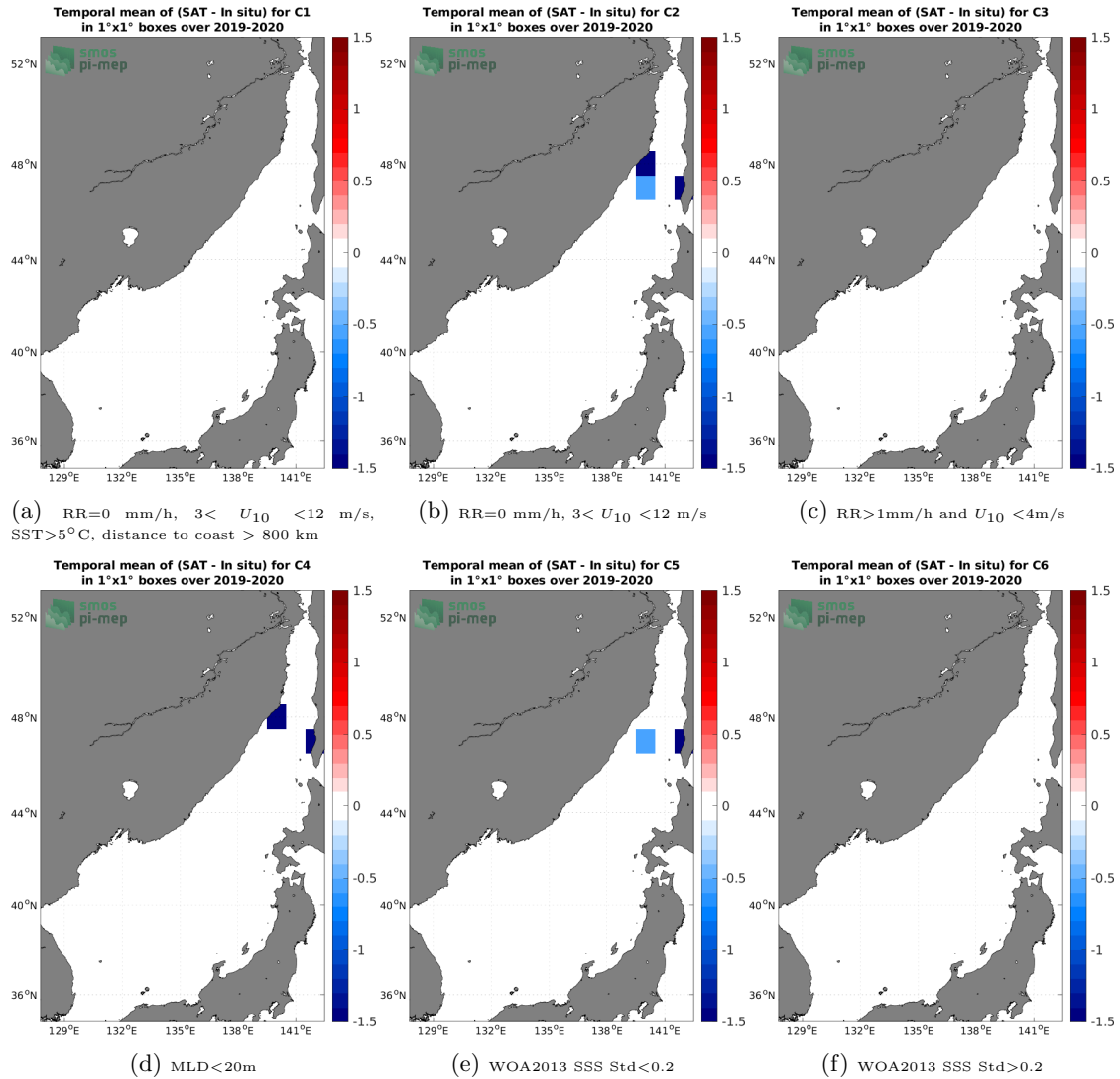
Figure 12: Temporal mean gridded over spatial boxes of size 1^\circ \times 1^\circ of \Delta\text{SSS} (SMOS SSS L2 v700 (ESA) - Argo) for 6 different subdatasets corresponding to: RR=0 mm/h, 3 < U_{10} < 12 m/s, SST > 5^\circ\text{C} , distance to coast > 800 km (a), RR=0 mm/h, 3 < U_{10} < 12 m/s (b), RR > 1 mm/h and U_{10} < 4 m/s (c), MLD < 20 m (d), WOA2013 SSS Std < 0.2 (e), WOA2013 SSS Std > 0.2 (f).
