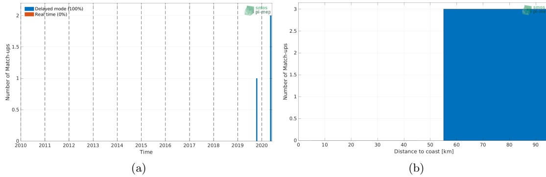
Figure 1: Number of match-ups between Argo and SMOS SSS L2 v700 (ESA) SSS as a function of time (a) and as function of the distance to coast (b) over the Sea of Japan Pi-MEP region and for the full satellite product period.
