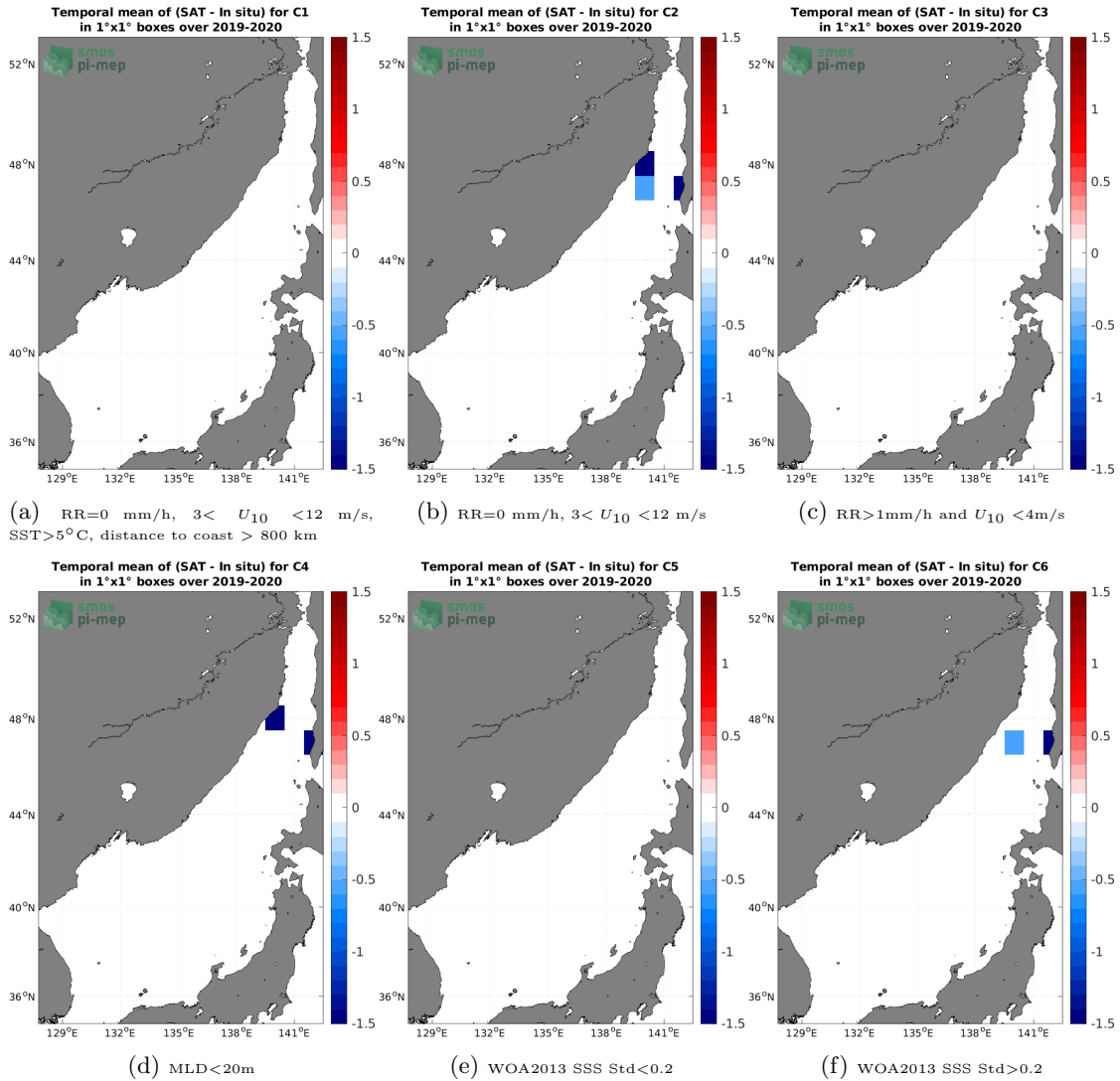
Figure 12: Temporal mean gridded over spatial boxes of size 1^\circ \times 1^\circ of \Delta SSS (SMOS SSS L2 v700 (ESA) - Argo) for 6 different subdatasets corresponding to: RR=0 mm/h, 3 < U_{10} < 12 m/s, SST > 5°C, distance to coast > 800 km (a), RR=0 mm/h, 3 < U_{10} < 12 m/s (b), RR > 1mm/h and U_{10} < 4 m/s (c), MLD < 20m (d), WOA2013 SSS Std < 0.2 (e), WOA2013 SSS Std > 0.2 (f).
