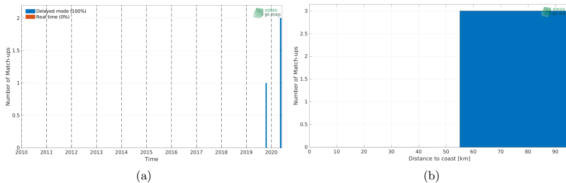
Figure 1: Number of match-ups between Argo and SMOS SSS L2 v700 (ESA) SSS as a function of time (a) and as function of the distance to coast (b) over the Sea of Japan Pi-MEP region and for the full satellite product period.
