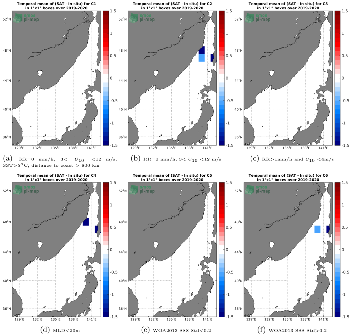
Figure 12: Temporal mean gridded over spatial boxes of size 1^\circ \times 1^\circ of \Delta SSS (SMOS SSS L2 v700 (ESA) - Argo) for 6 different subdatasets corresponding to:RR=0 mm/h, 3 < U_{10} < 12 m/s, SST>5°C, distance to coast > 800 km (a), RR=0 mm/h, 3 < U_{10} < 12 m/s (b), RR>1mm/h and U_{10} < 4 m/s (c),MLD<20m (d),WOA2013 SSS Std<0.2 (e),WOA2013 SSS Std>0.2 (f).
