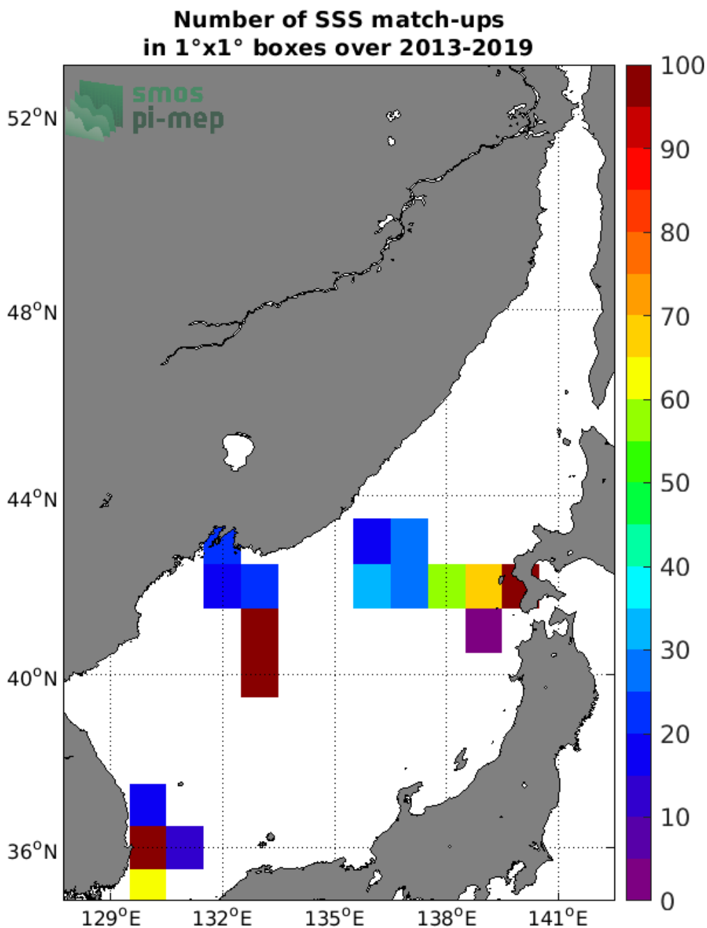
Figure 4: Number of SSS match-ups between TSG (LEGOS-DM) SSS and the SMOS SSS L2 v662 (ESA) SSS product for the Sea of Japan Pi-MEP region over 1°x1° boxes and for the full satellite product period.
