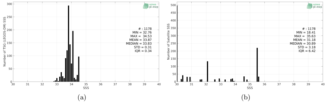
Figure 2: Histograms of SSS from TSG (LEGOS-DM) (a) and SMOS SSS L2 v662 (ESA) (b) considering all match-up pairs per bins of 0.1 over the Sea of Japan Pi-MEP region and for the full satellite product period.
