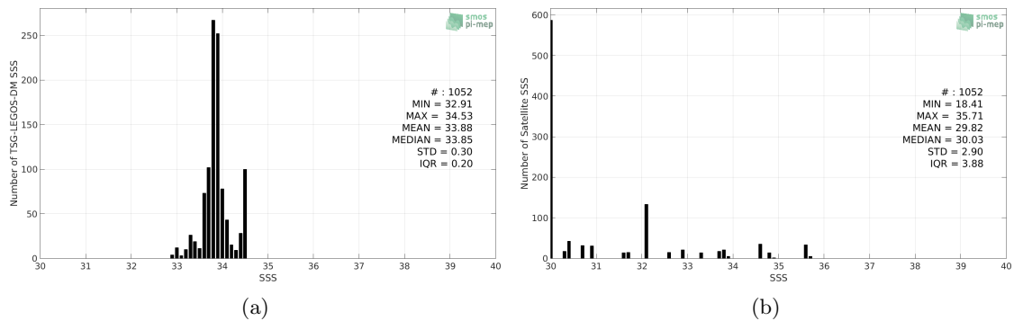
Figure 2: Histograms of SSS from TSG-LEGOS-DM (a) and SMOS L2 v662 (ESA) (b) considering all match-up pairs per bins of 0.1 over the Sea of Japan Pi-MEP region and for the full satellite product period.
