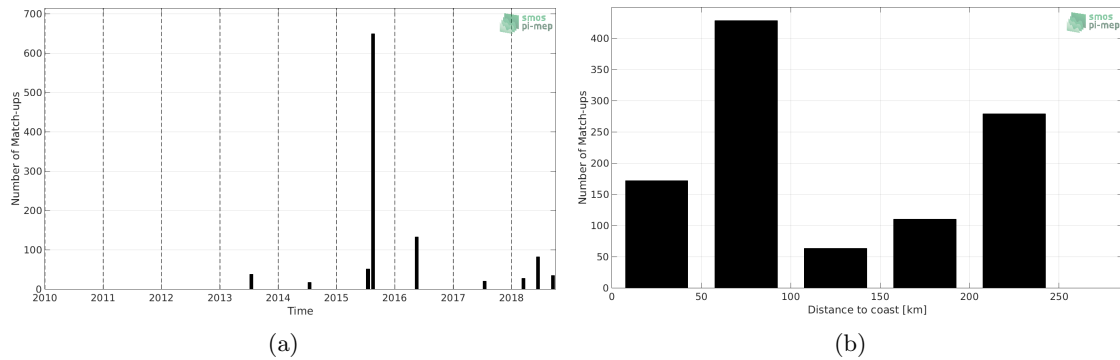
Figure 1: Number of match-ups between TSG-LEGOS-DM and SMOS L2 v662 (ESA) SSS as a function of time (a) and as function of the distance to coast (b) over the Sea of Japan Pi-MEP region and for the full satellite product period.
