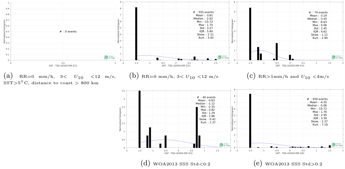
Figure 13: Normalized histogram of \Delta\text{SSS} (SMOS L2 v662 (ESA) - TSG-LEGOS-DM) for 5 different subdatasets corresponding to: RR=0 mm/h, 3 < U_{10} < 12 m/s, SST > 5^\circ\text{C} , distance to coast > 800 km (a), RR=0 mm/h, 3 < U_{10} < 12 m/s (b), RR > 1\text{mm/h} and U_{10} < 4\text{m/s} (c), WOA2013 SSS Std < 0.2 (d), WOA2013 SSS Std > 0.2 (e).
