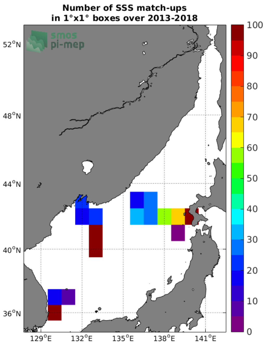
Figure 4: Number of SSS match-ups between TSG-LEGOS-DM SSS and the SMOS L2 v662 (ESA) SSS product for the Sea of Japan Pi-MEP region over 1°x1° boxes and for the full satellite product period.
