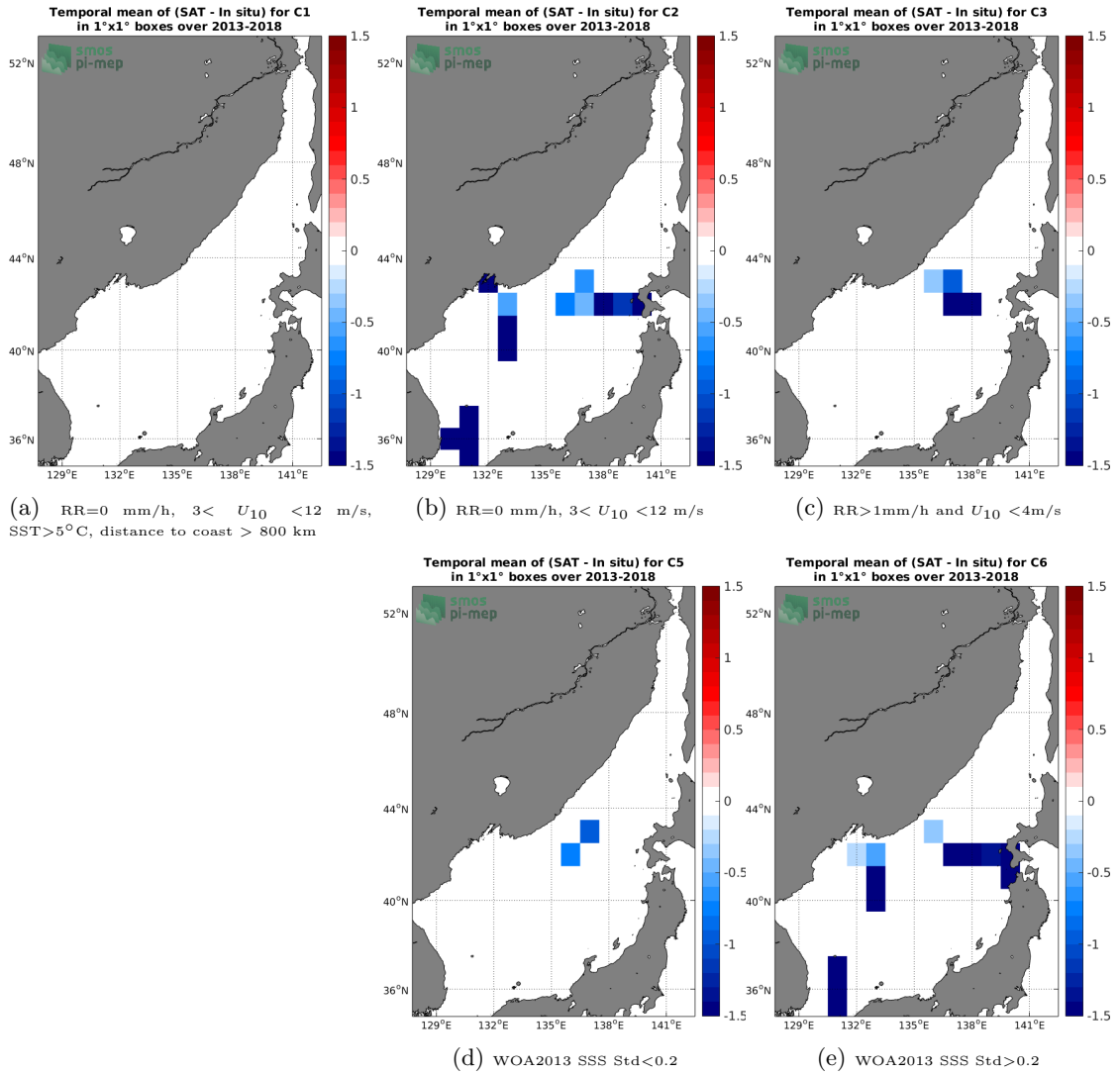
Figure 12: Temporal mean gridded over spatial boxes of size 1°x1° of \Delta SSS (SMOS L2 v662 (ESA) - TSG-LEGOS-DM) for 5 different subdatasets corresponding to:RR=0 mm/h, 3 < U_{10} < 12 m/s, SST>5°C, distance to coast > 800 km (a), RR=0 mm/h, 3 < U_{10} < 12 m/s (b), RR>1mm/h and U_{10} < 4 m/s (c), WOA2013 SSS Std<0.2 (d), WOA2013 SSS Std>0.2 (e).
