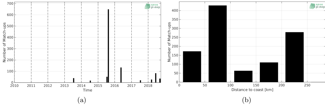
Figure 1: Number of match-ups between TSG-LEGOS-DM and SMOS-L2-DPGS-v662 SSS as a function of time (a) and as function of the distance to coast (b) over the Sea of Japan Pi-MEP region and for the full satellite product period.
