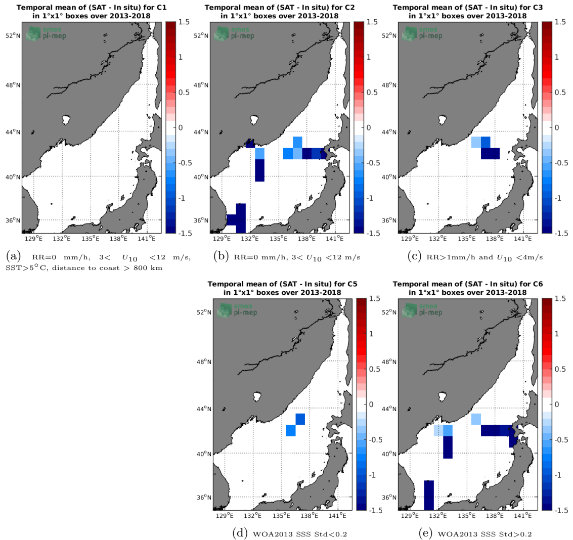
Figure 12: Temporal mean gridded over spatial boxes of size 1^\circ \times 1^\circ of \Delta SSS (SMOS-L2-DPGS-v662 - TSG-LEGOS-DM) for 5 different subdatasets corresponding to:RR=0 mm/h, 3 < U_{10} < 12 m/s, SST > 5^\circ\text{C} , distance to coast > 800 km (a), RR=0 mm/h, 3 < U_{10} < 12 m/s (b), RR > 1 mm/h and U_{10} < 4 m/s (c), WOA2013 SSS Std < 0.2 (d), WOA2013 SSS Std > 0.2 (e).
