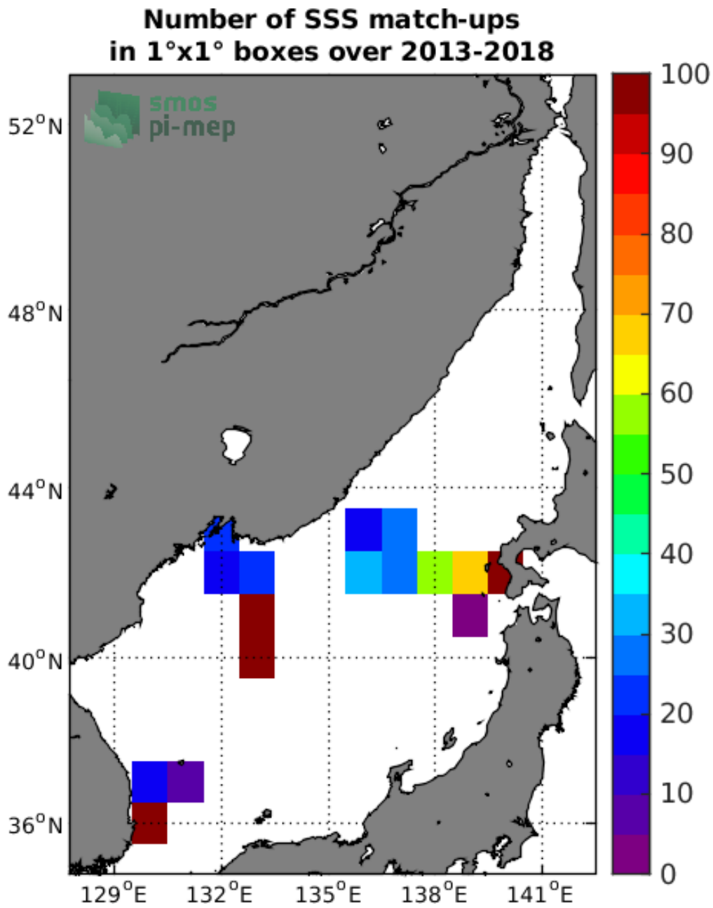
Figure 4: Number of SSS match-ups between TSG-LEGOS-DM SSS and the SMOS-L2-DPGS-v662 SSS product for the Sea of Japan Pi-MEP region over 1°x1° boxes and for the full satellite product period.
