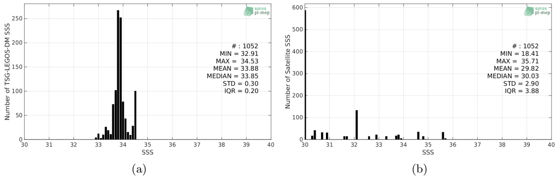
Figure 2: Histograms of SSS from TSG-LEGOS-DM (a) and SMOS-L2-DPGS-v662 (b) considering all match-up pairs per bins of 0.1 over the Sea of Japan Pi-MEP region and for the full satellite product period.
