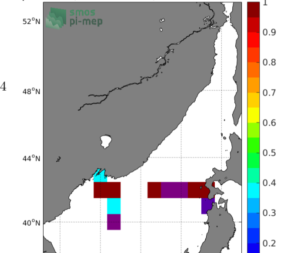
Temporal STD of (Sat-TSG-LEGOS-DM) in 1°x1° boxes over 2013-2017
