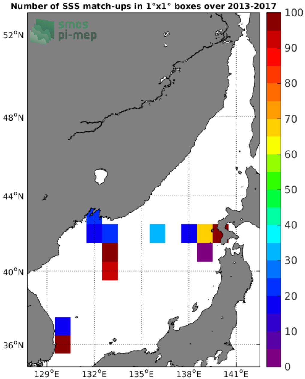
Figure 4: Number of SSS match-ups between TSG-LEGOS-DM SSS and the SMOS-L2-DPGS-v662 SSS product for the Sea of Japan Pi-MEP region over 1°x1° boxes and for the full satellite product period.
