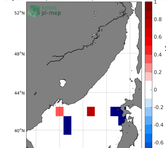
Temporal mean of (Sat-TSG-LEGOS-DM) in 1°x1° boxes over 2013-2016
