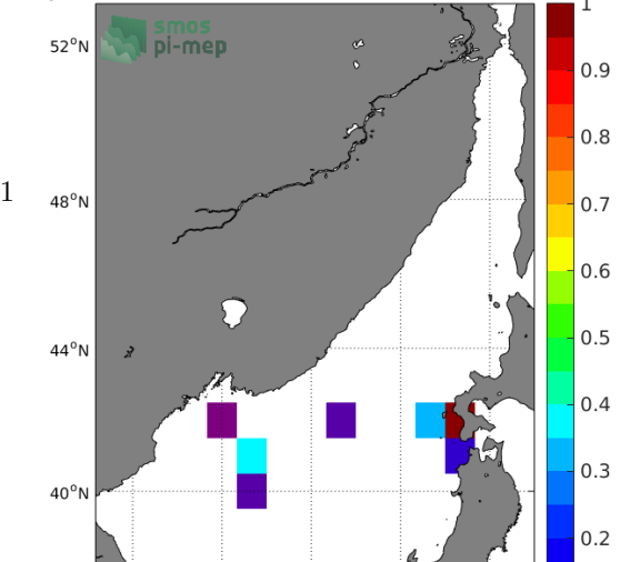
Temporal STD of (Sat-TSG-LEGOS-DM) in 1°x1° boxes over 2013-2016
