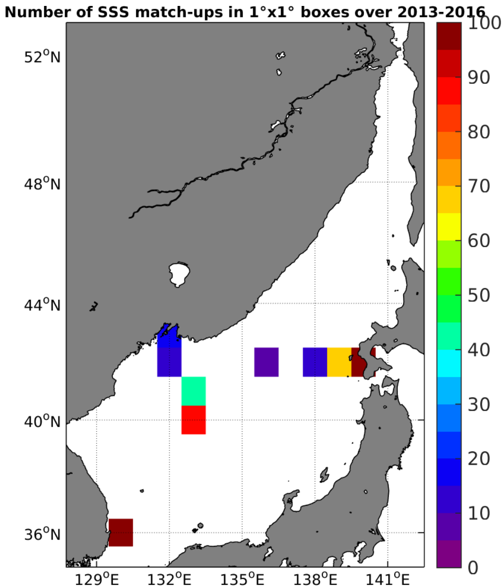
Figure 4: Number of SSS match-ups between TSG-LEGOS-DM SSS and the SMOS-L2-DPGS-v662 SSS product for the Sea of Japan Pi-MEP region over 1°x1° boxes and for the full satellite product period.
