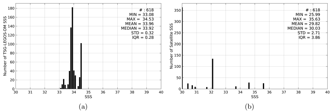
Figure 2: Histograms of SSS from TSG-LEGOS-DM (a) and SMOS-L2-DPGS-v662 (b) considering all match-up pairs per bins of 0.1 over the Sea of Japan Pi-MEP region and for the full satellite product period.
