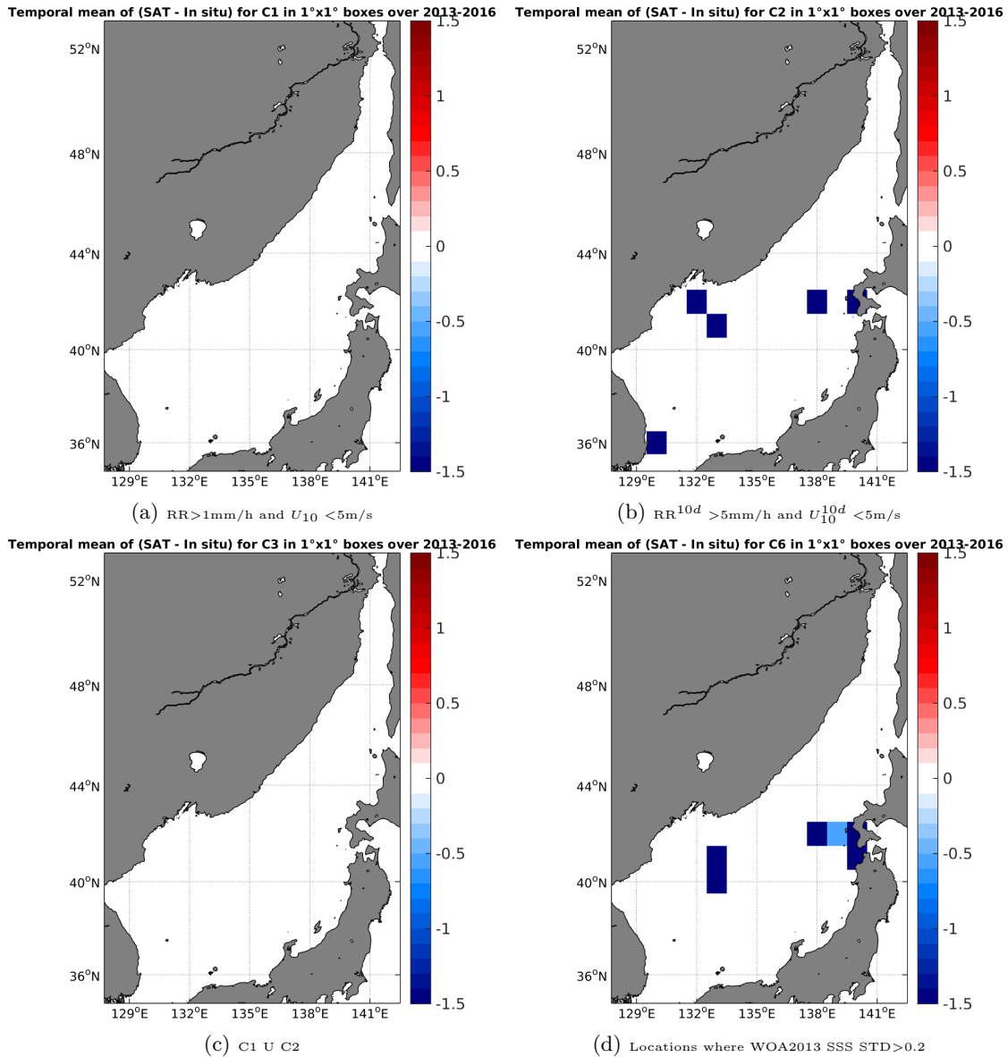
Figure 12: Temporal mean gridded over spatial boxes of size 1°x1° of \Delta SSS (SMOS-L2-DPGS-v662 - TSG-LEGOS-DM) for 4 different subdatasets corresponding to: RR > 1\text{mm/h} and U_{10} < 5\text{m/s} (a), RR^{10d} > 5\text{mm/h} and U_{10}^{10d} < 5\text{m/s} (b), C1 U C2 (c), Locations where WOA2013 SSS STD > 0.2 (d).
