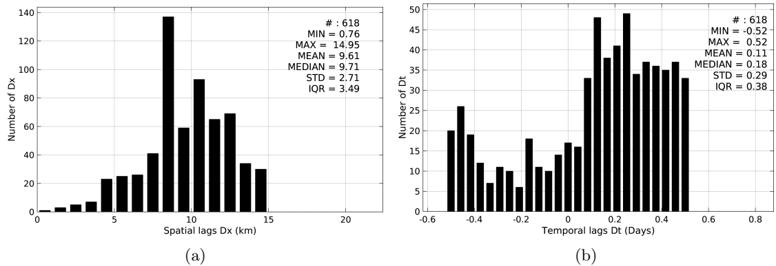
Figure 5: Histograms of the spatial (a) and temporal (b) lags between the time of the TSG-LEGOS-DM measurements and the date of the corresponding SMOS-L2-DPGS-v662 SSS product.
