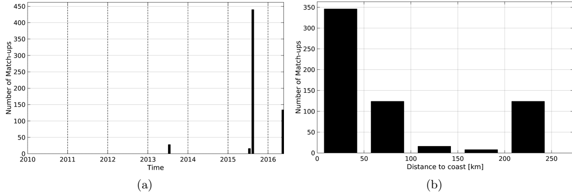
Figure 1: Number of match-ups between TSG-LEGOS-DM and SMOS-L2-DPGS-v662 SSS as a function of time (a) and as function of the distance to coast (b) over the Sea of Japan Pi-MEP region and for the full satellite product period.
