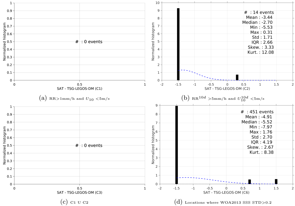
Figure 13: Normalized histogram of \Delta\text{SSS} (SMOS-L2-DPGS-v662 - TSG-LEGOS-DM) for 6 different subdatasets corresponding to: RR > 1\text{mm/h} and U_{10} < 5\text{m/s} (a), RR^{10d} > 5\text{mm/h} and U_{10}^{10d} < 5\text{m/s} (b), C1 U C2 (c), Locations where WOA2013 SSS STD > 0.2 (d).
