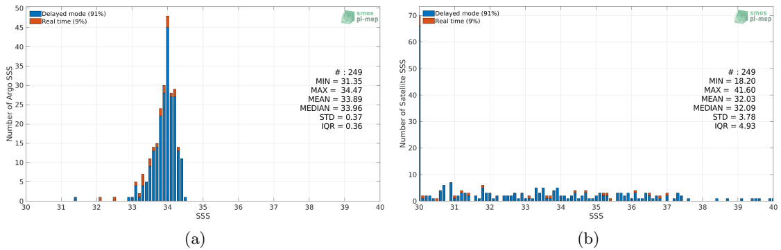
Figure 2: Histograms of SSS from Argo (a) and SMOS SSS L2 v662 (ESA) (b) considering all match-up pairs per bins of 0.1 over the Sea of Japan Pi-MEP region and for the full satellite product period.
