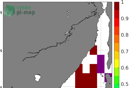
Temporal STD of (Sat - Argo) in 1°x1° boxes over 2013-2021
