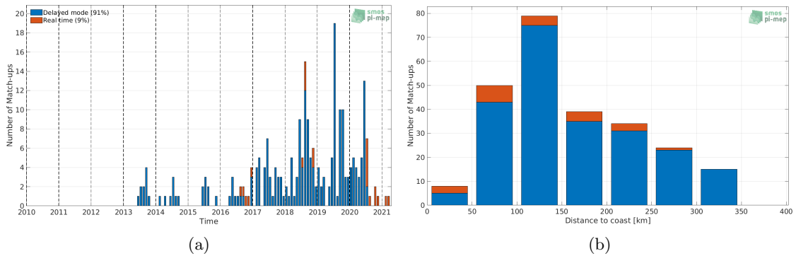
Figure 1: Number of match-ups between Argo and SMOS SSS L2 v662 (ESA) SSS as a function of time (a) and as function of the distance to coast (b) over the Sea of Japan Pi-MEP region and for the full satellite product period.
