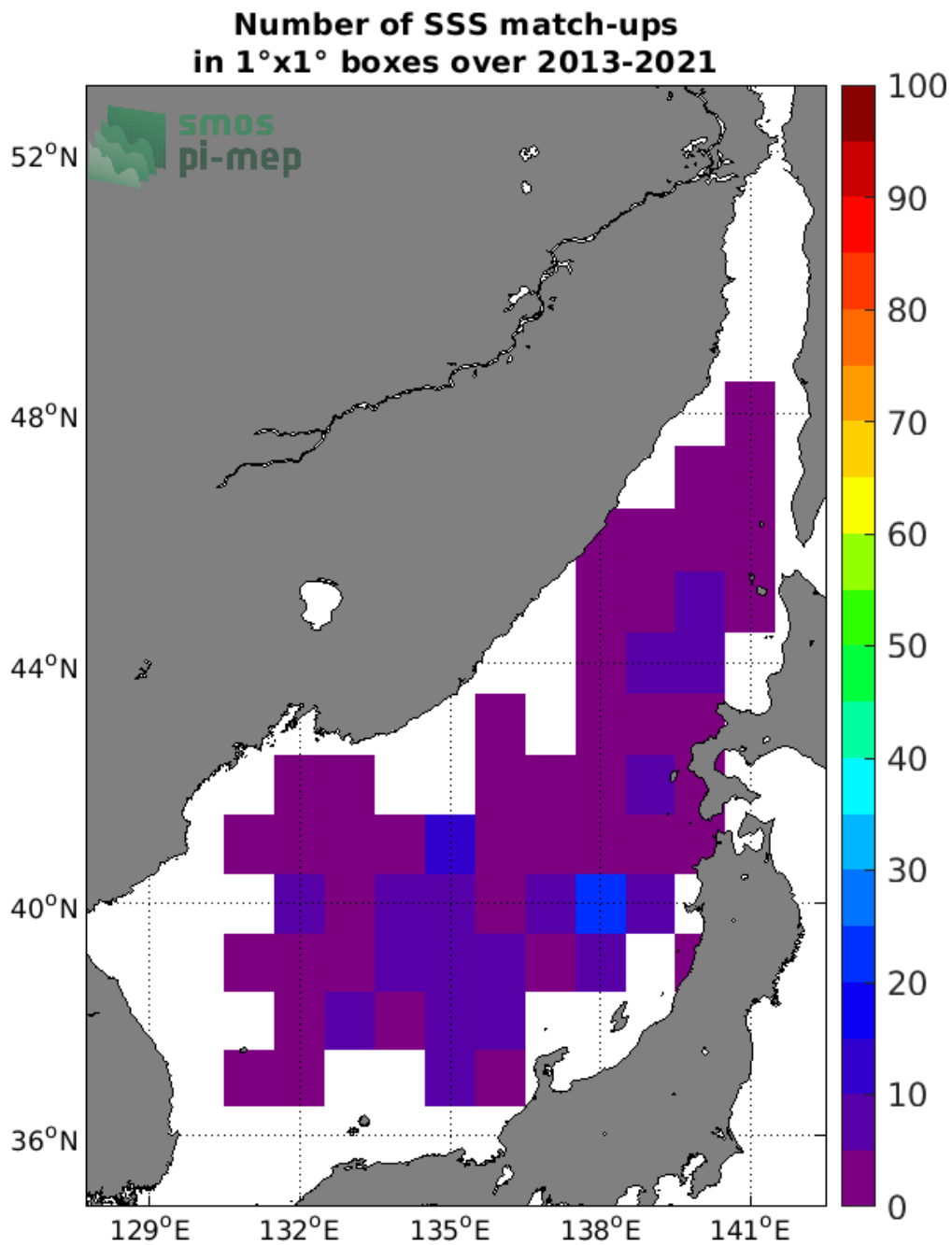
Figure 4: Number of SSS match-ups between Argo SSS and the SMOS SSS L2 v662 (ESA) SSS product for the Sea of Japan Pi-MEP region over 1°x1° boxes and for the full satellite product period.
